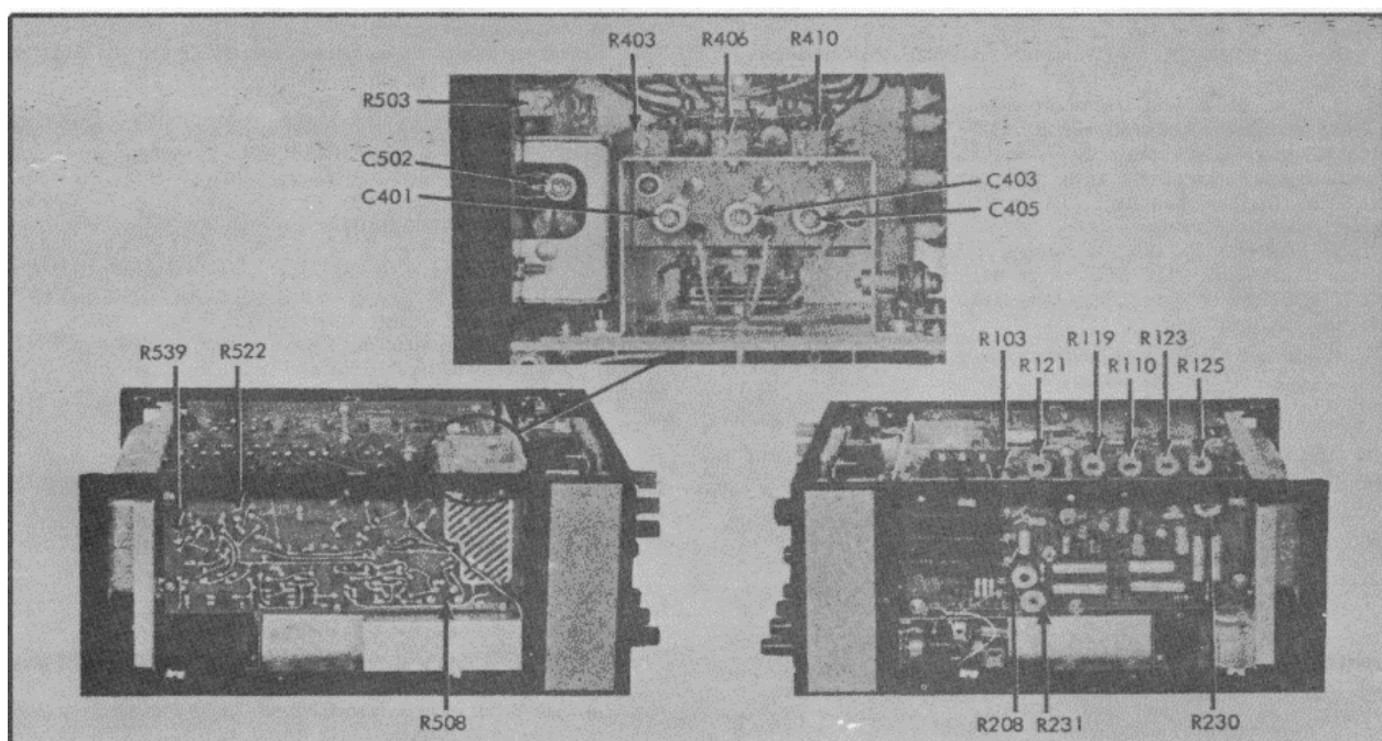
Figure 4-8. ADJUSTMENT LOCATIONS
