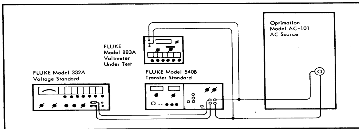
Figure 4-6. AC TO DC CONVERTER CALIBRATION SETUP
