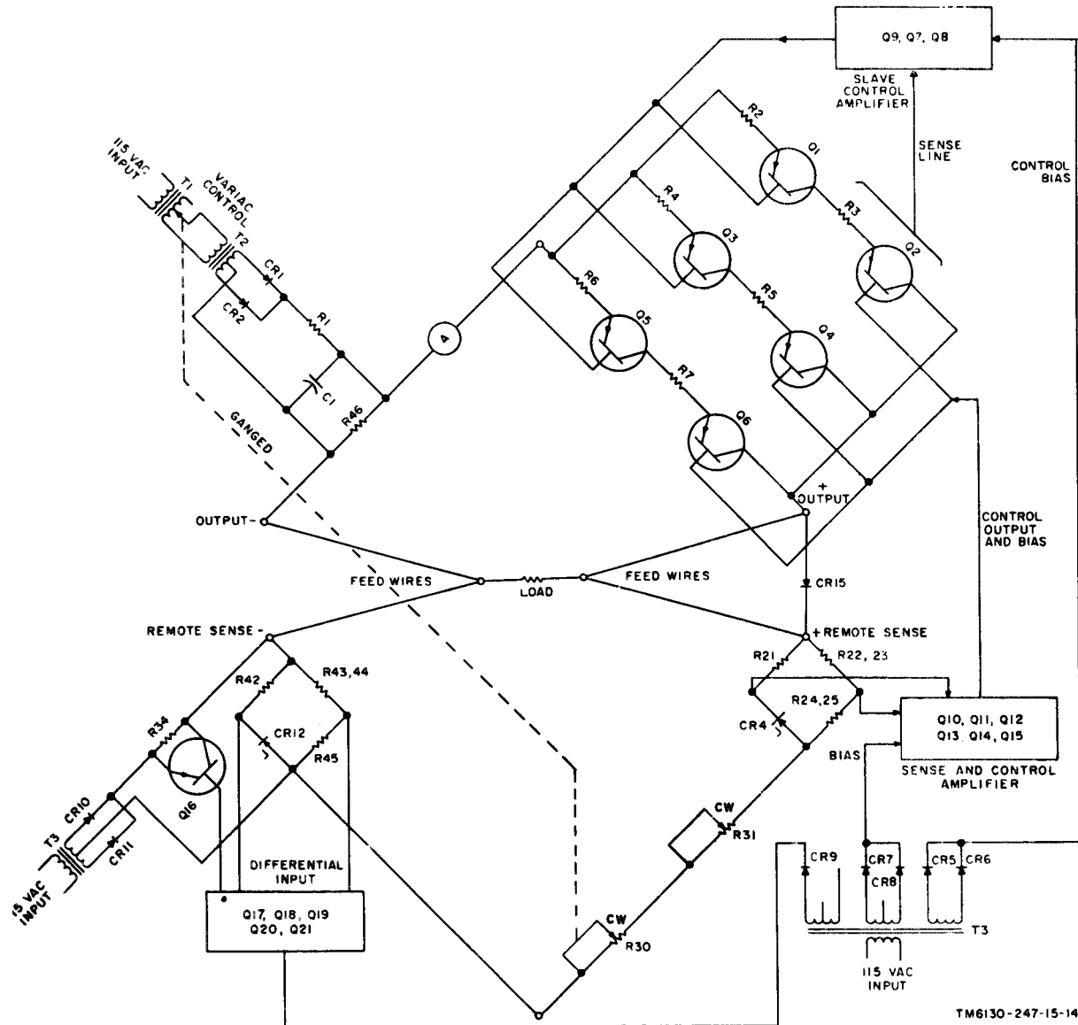
4-3. Detailed Function of Main Control Amplifier (fig. 4-3)
