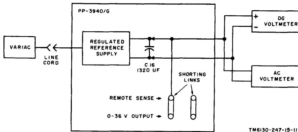
Figure 6-2. Connections for reference supply tests.
