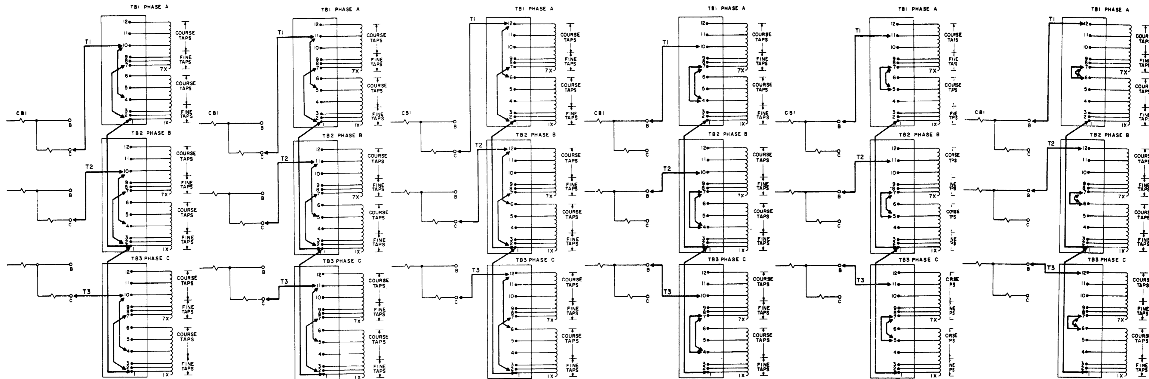
A. 198-VOLT POWER CONNECTIONS
