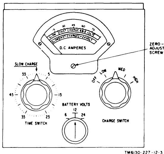
Figure 3. PP-1 660/G, operator's controls and indicator.
