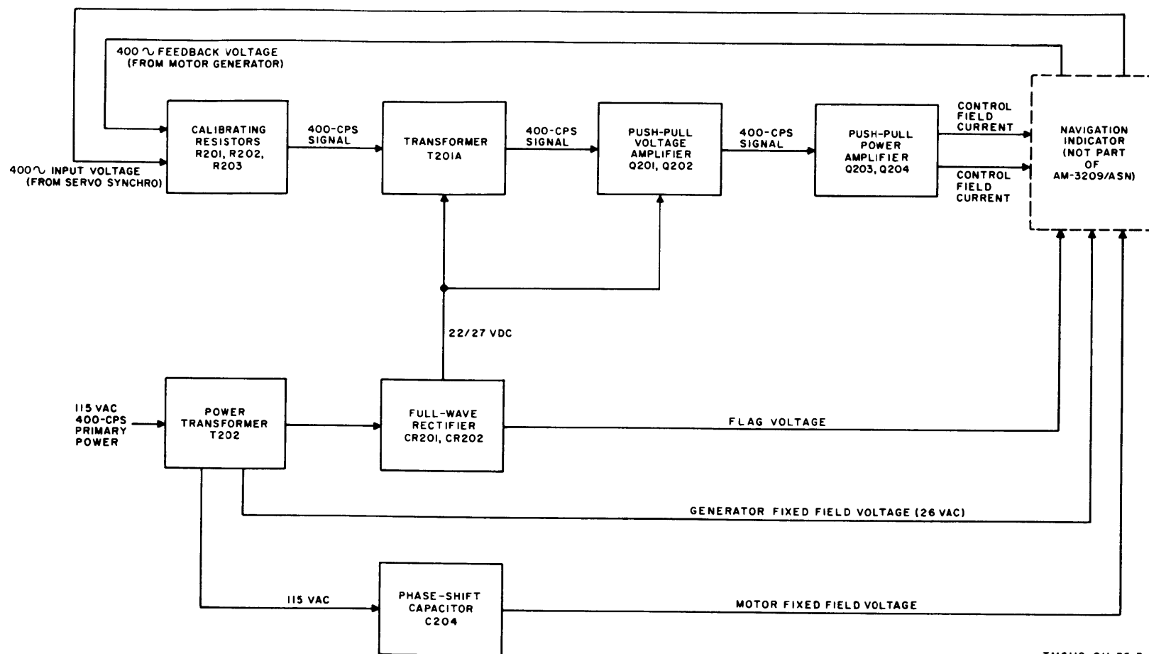
Figure 2-1. Amplifier, Electronic Control AM-3209/ASN, block diagram.
