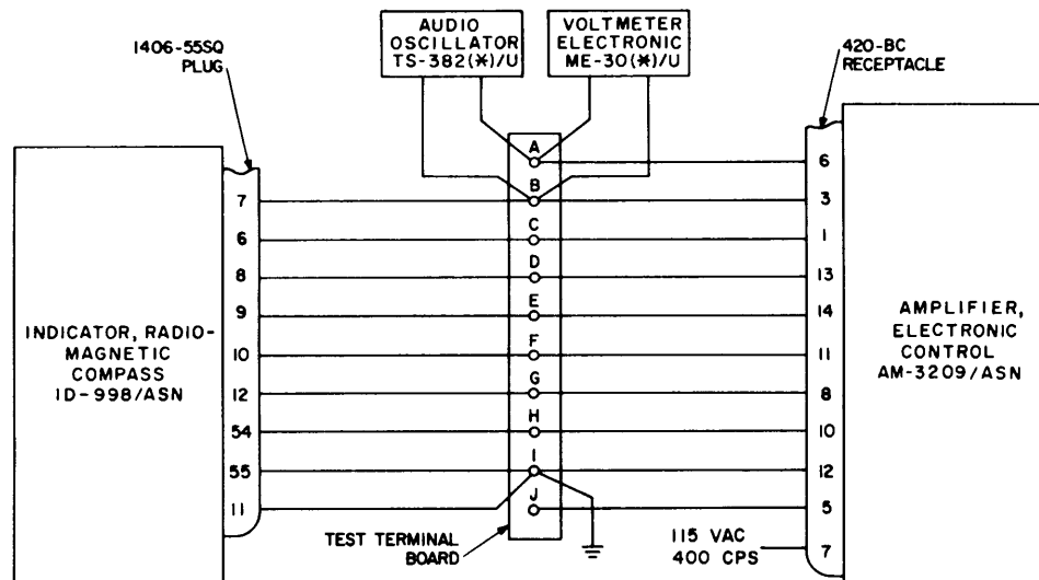
Figure 3-3. Amplifier, Electronic Control AM-3209/ASN, test setup.
