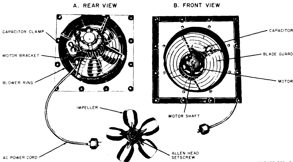
Figure 30. Exhaust blower, front and rear view.
