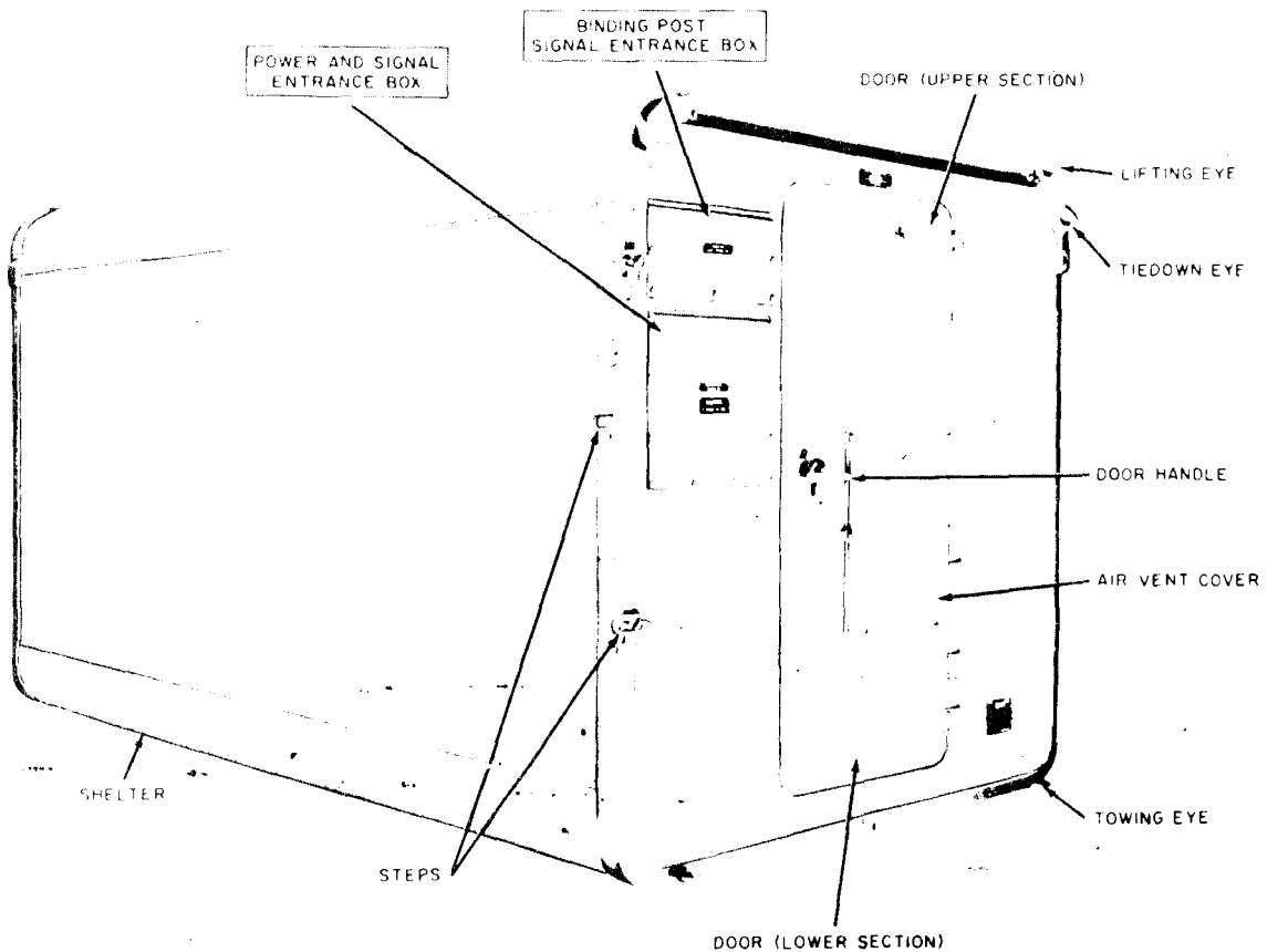
Figure 5. Operations Center, Communications AN/MS-31..
