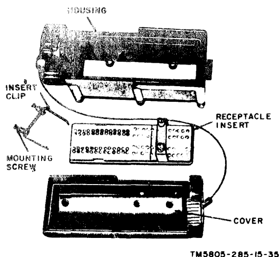
Figure 34. Cable receptacle, 26-pair, partially disassembled.
