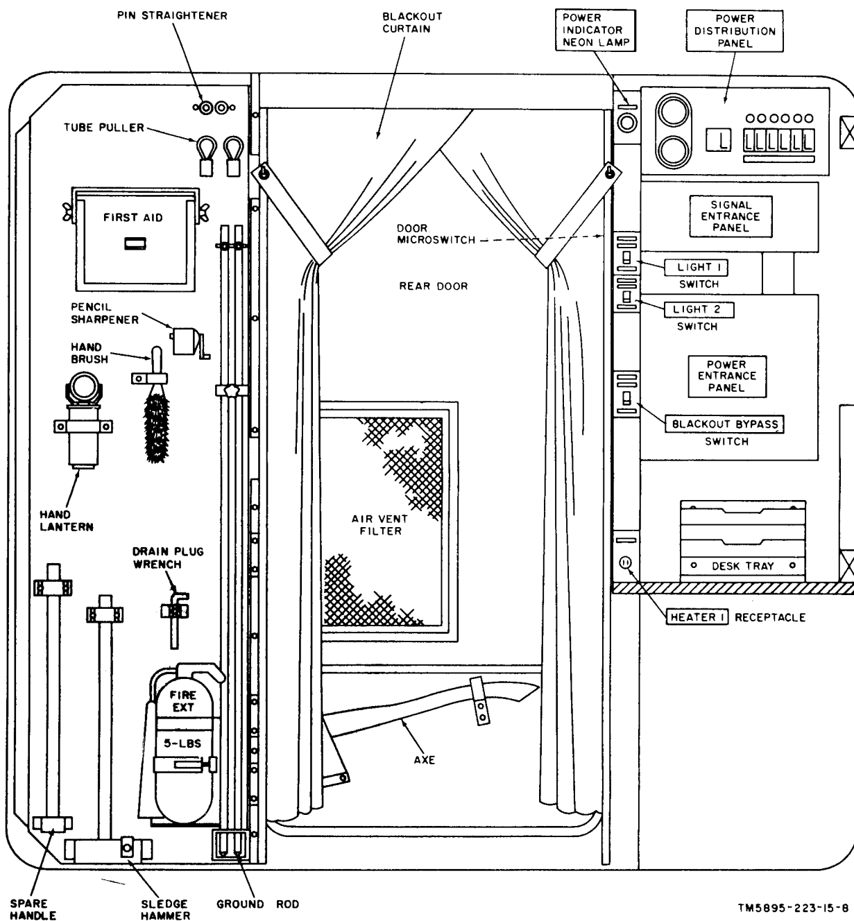
Figure 14. Operations Center, Communications AN/MS-31, rear wall, elevation diagram.
