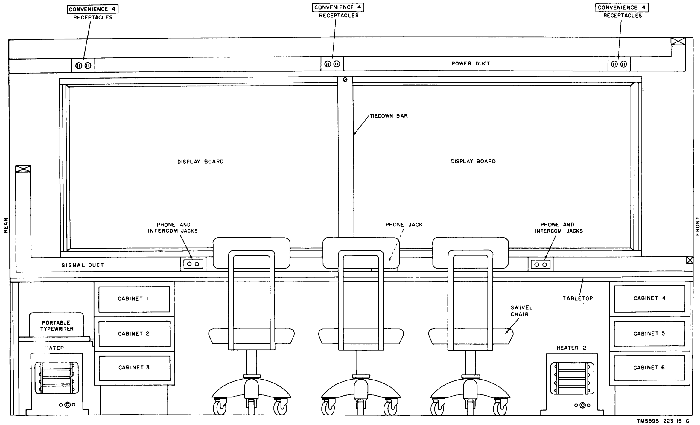
Figure 12. Operations Center, Communications AN/MSC-31, roadside wall, elevation diagram.
