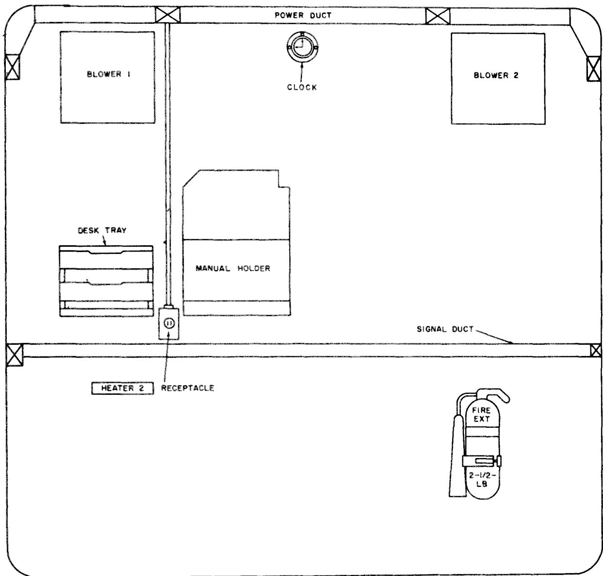
Figure 13. Operations Center, Communications AN/MS-31, front wall, elevation diagram.
