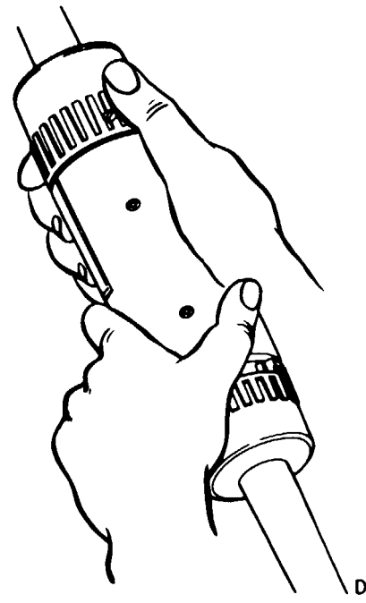
Figure 24. Coupling 26-pair connectors.
