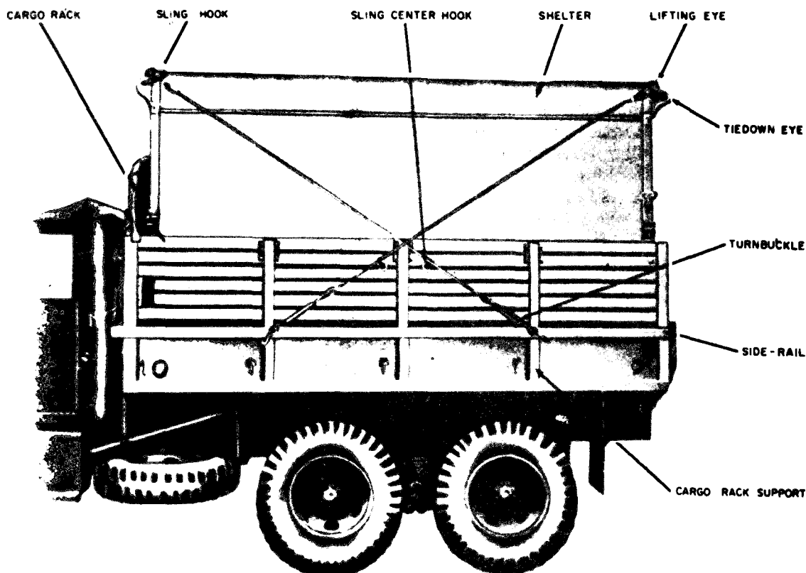
Figure 23. Securing AN/MS-31 on truck.
