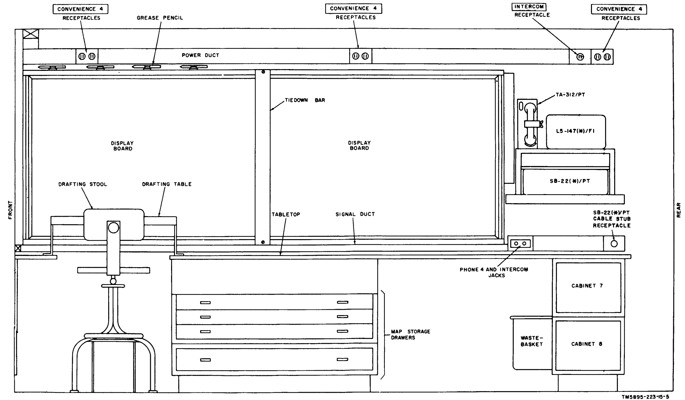
Figure 11. Operations Center, communications AN/MS-31, curbside wall, elevation diagram.
