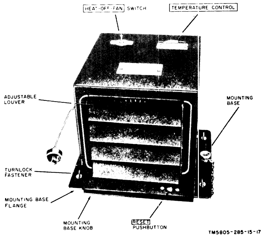
Figure 17. Electric heater.
