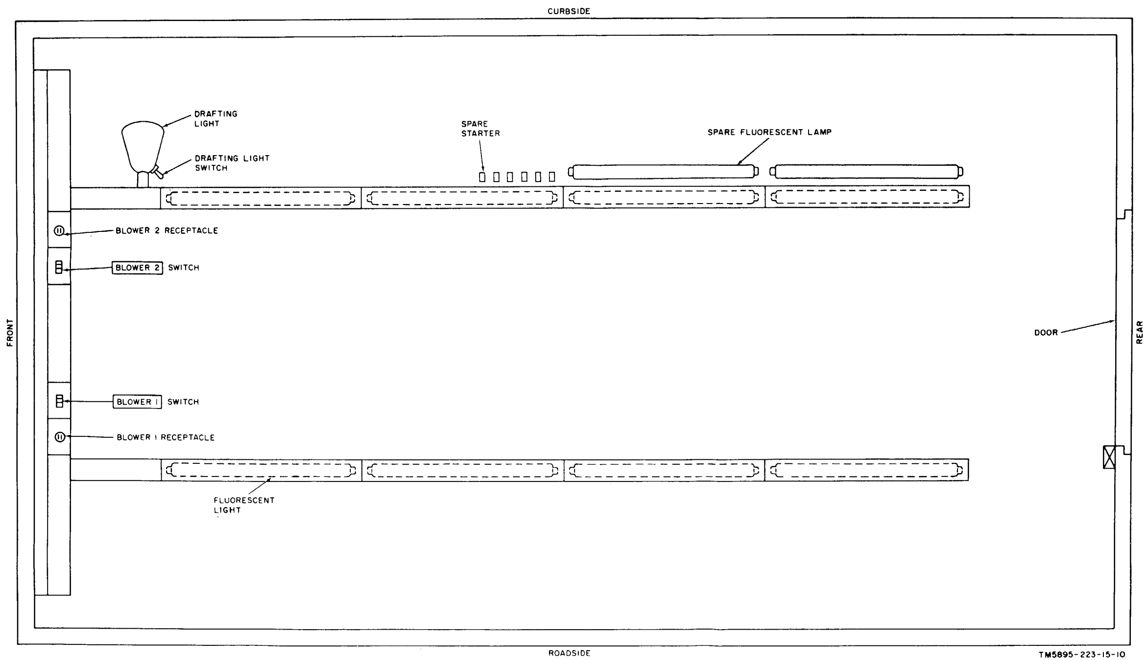
Figure 16. Operations Center, Communications AN/MSC-31, ceiling plan.
