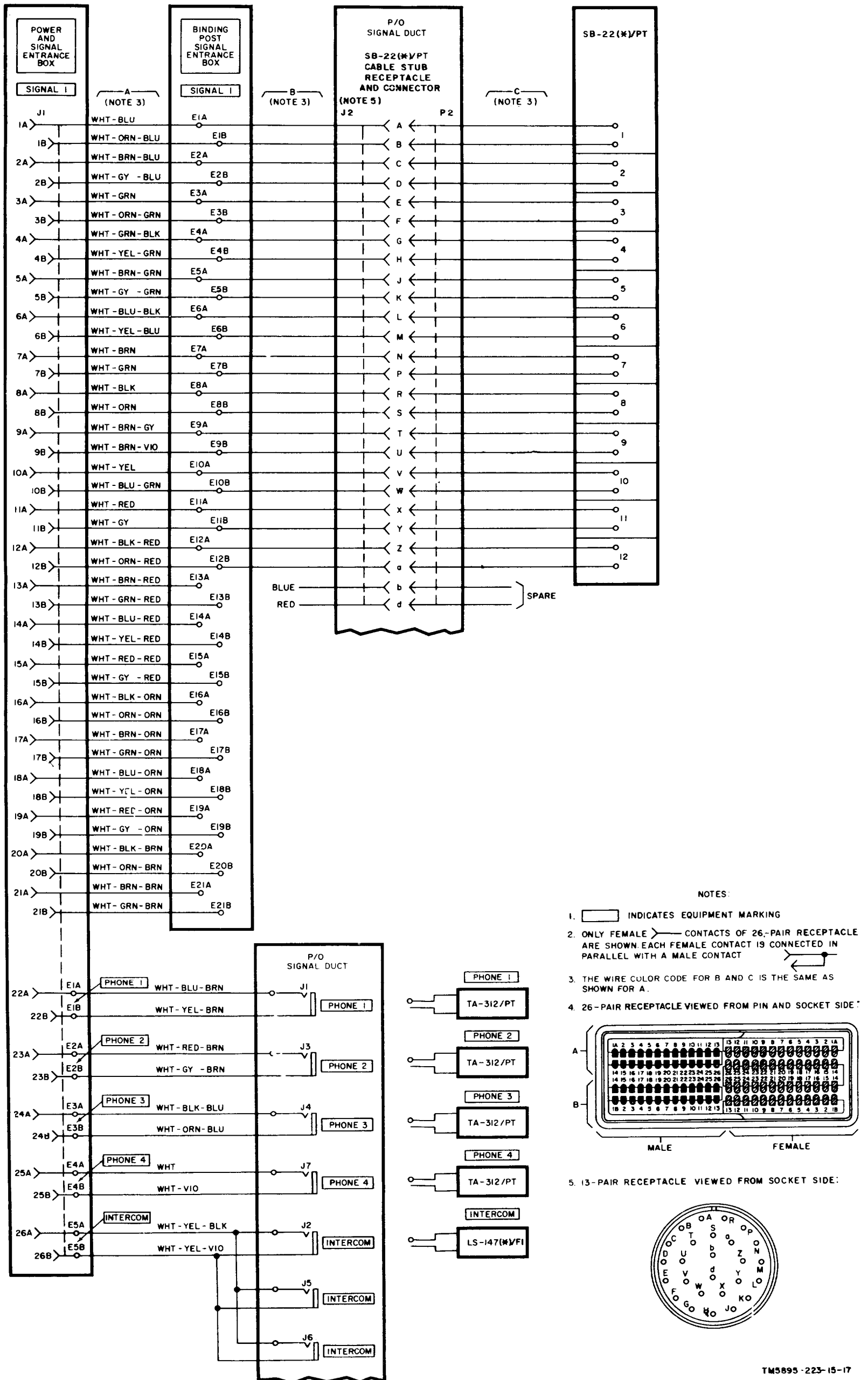
Figure 36. Operations Center, Communications AN/MSG-31, signal schematic-wiring diagram.
