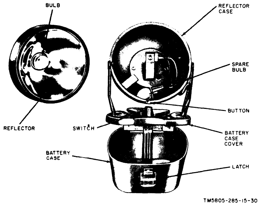
Figure 26. Hand lantern, partially disassembled.
