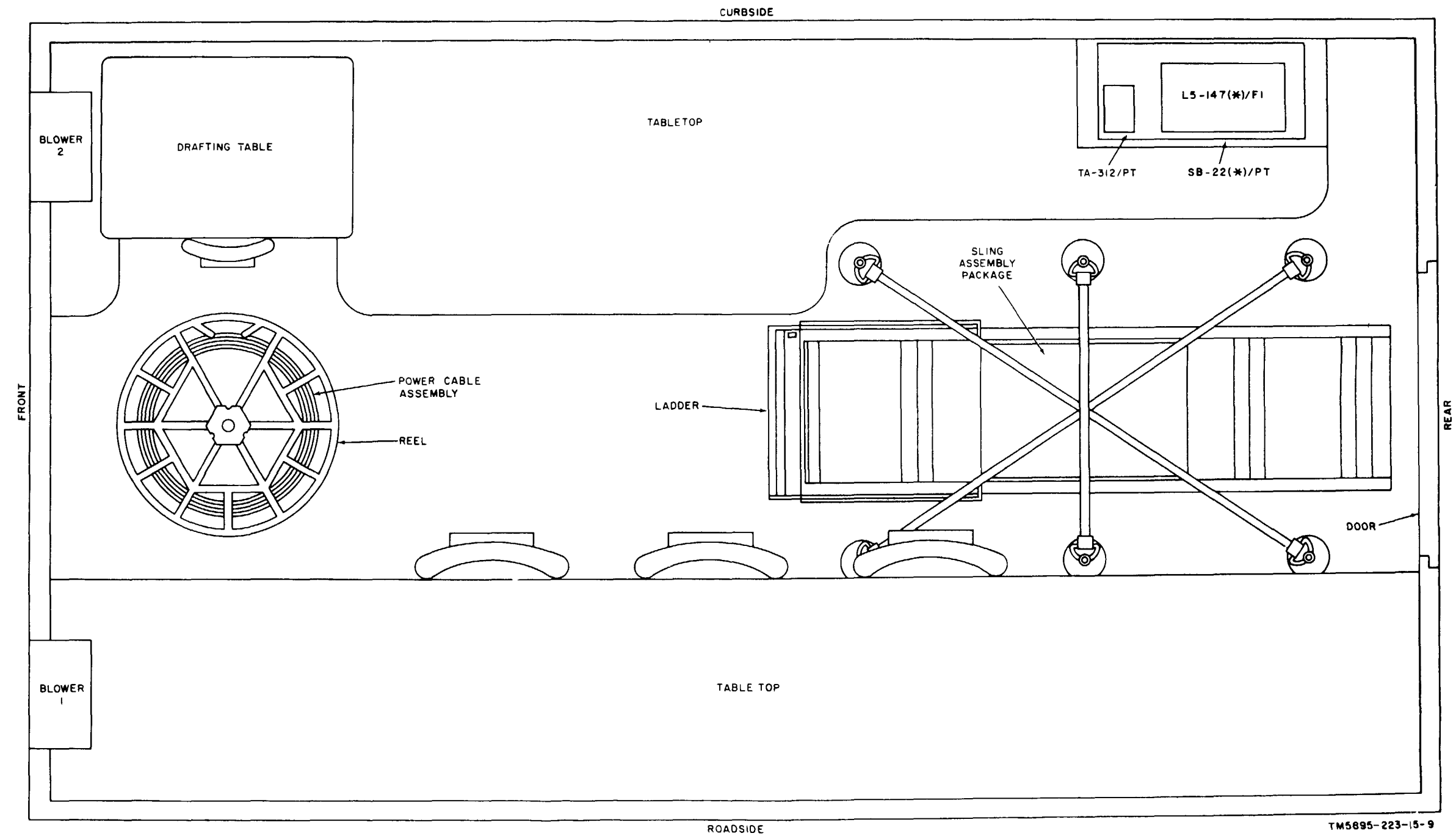
Figure 15. Operations Center, Communications AN/MSC-31, floor plan.
