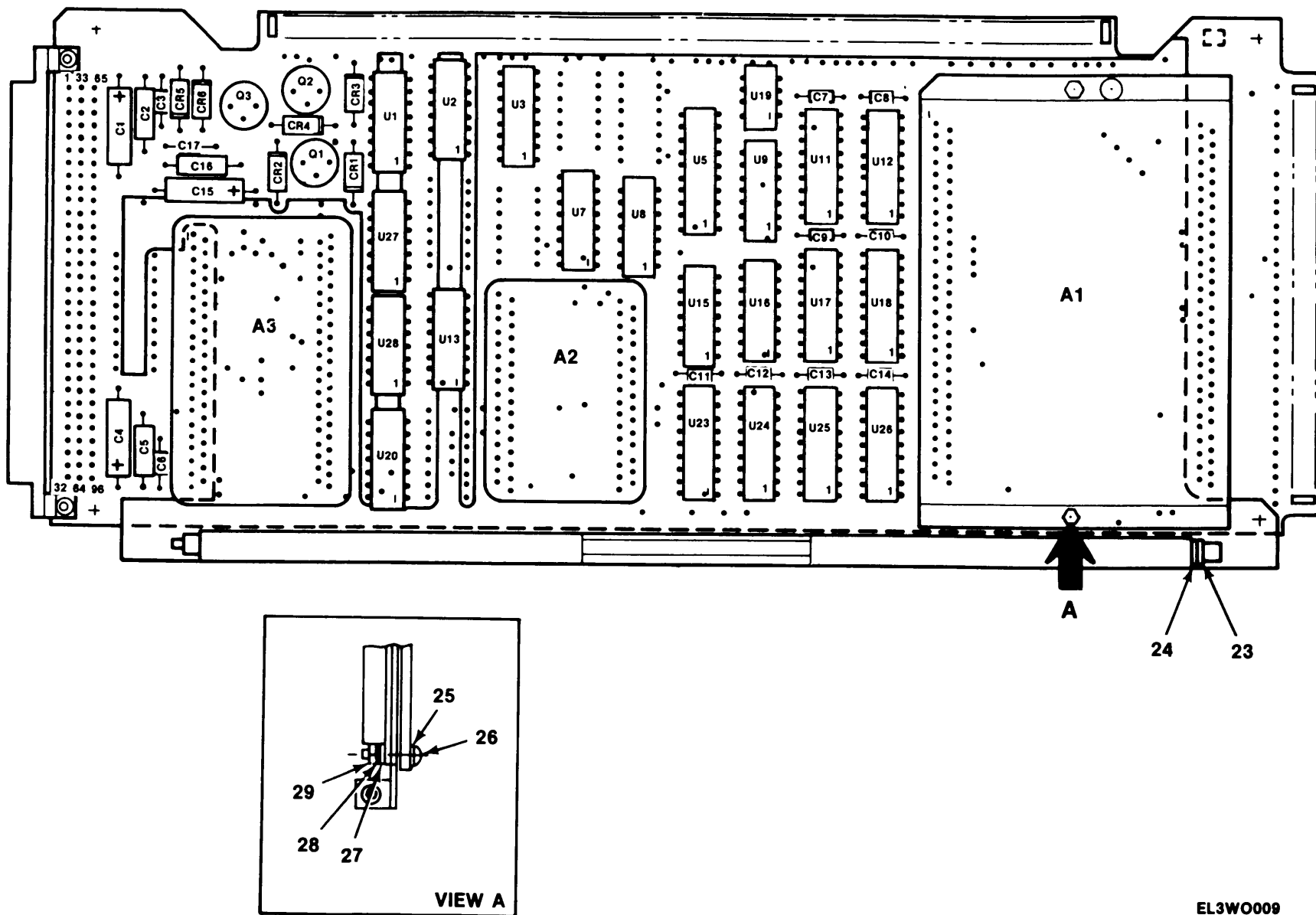
Figure 4. Circuit Card Assembly, SLO Processing (1A2) (Sheet 1 of 2)
