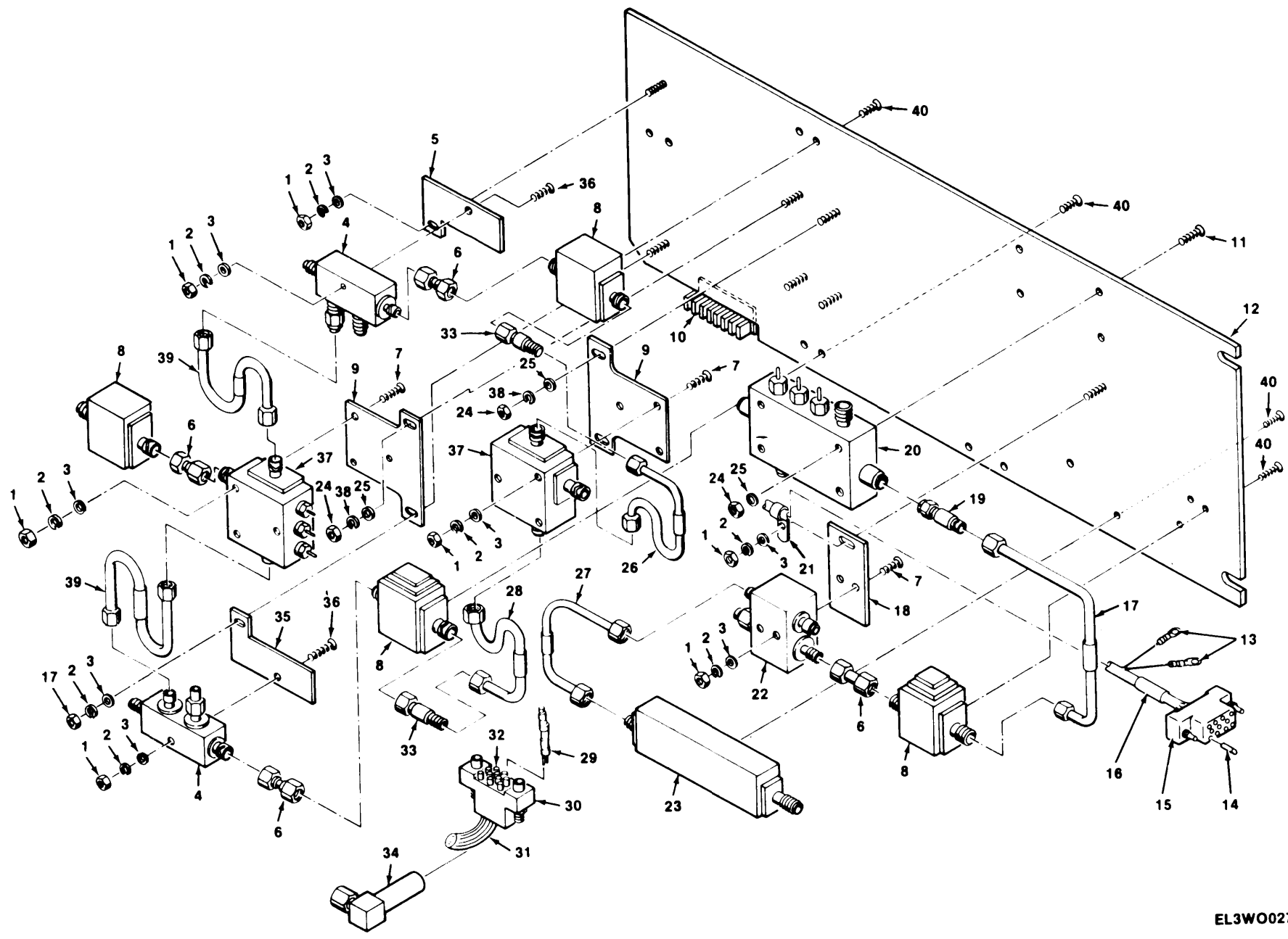
Figure 14. RF Tray Assembly
