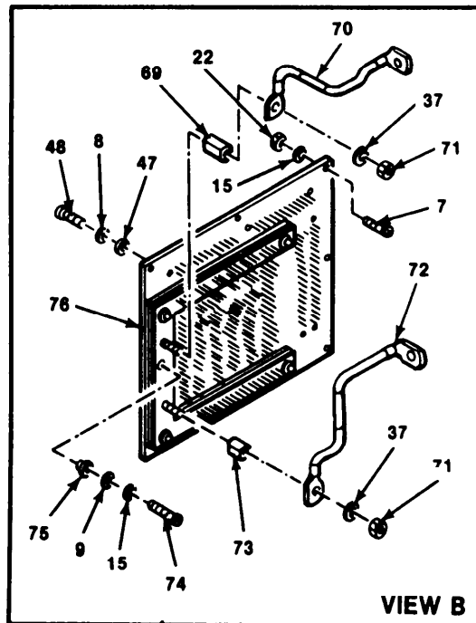
Figure 2. Receiver-Transmitter RT-1149(V)1/ALQ136(V) (Sheet 2 of 5).
