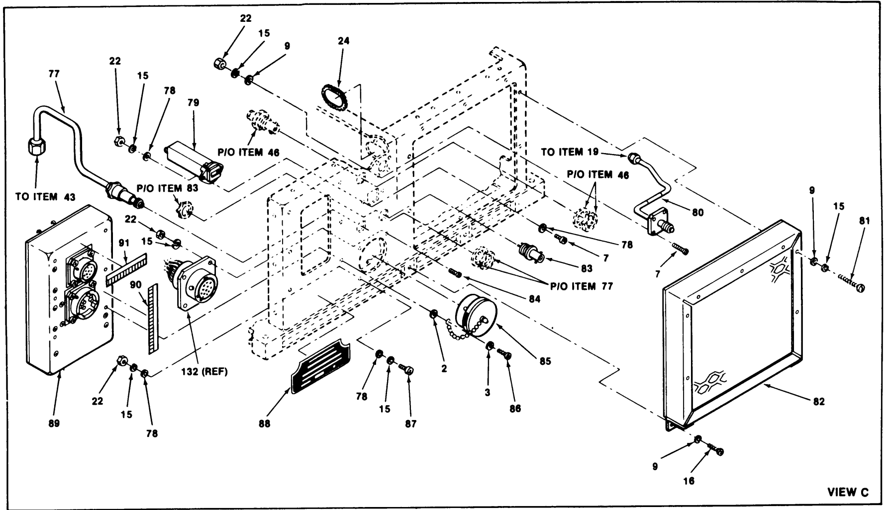
Figure 2. Receiver-Transmitter RT-1149(V)1/ALQ-136(V) (Sheet 3 of 5).
