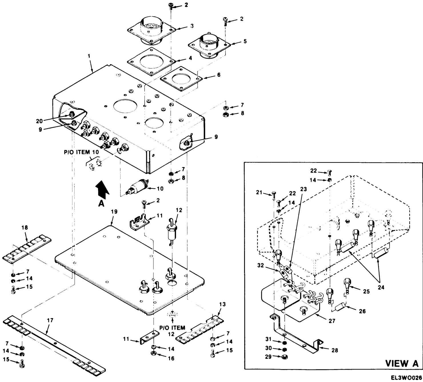
Figure 13. Filter Assembly
