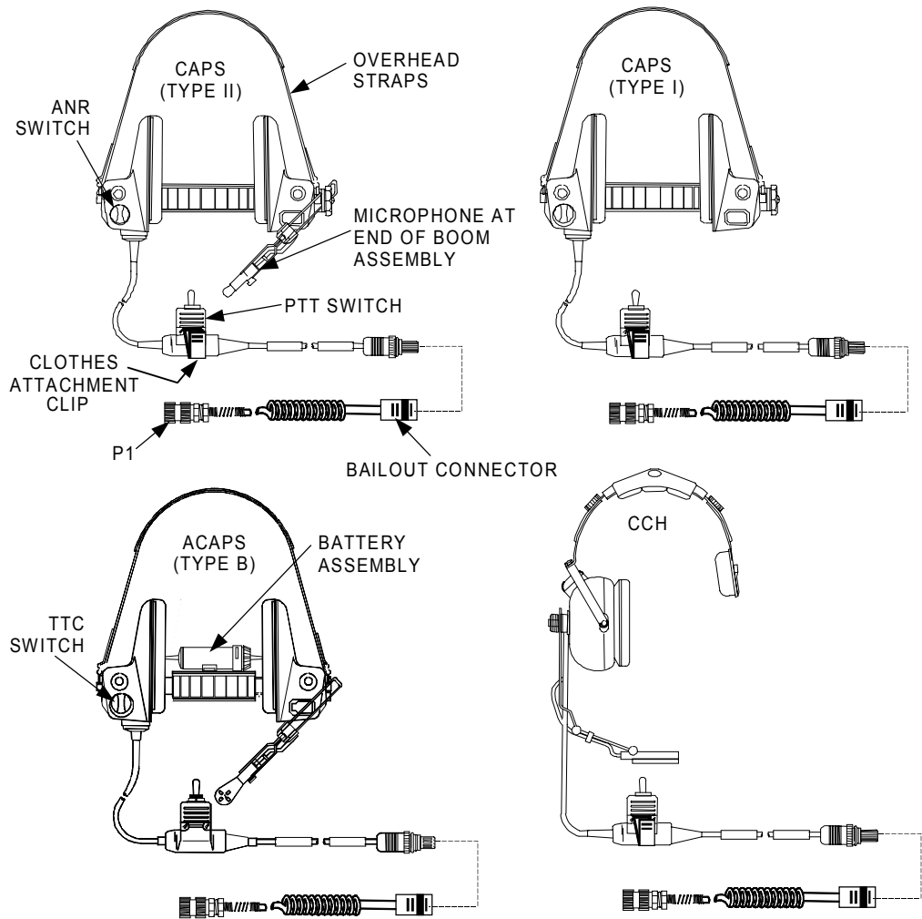
Figure 2-18. CAPS, ACAPS, and CCH Headsets Major Components
