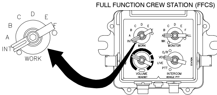
Figure 2-11. WORK Control Switch of FFCS
