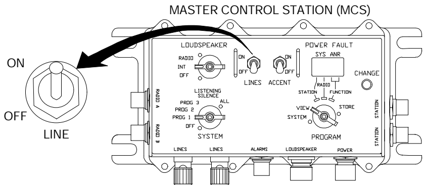
Figure 2-6. LINES Control Switch of MCS
