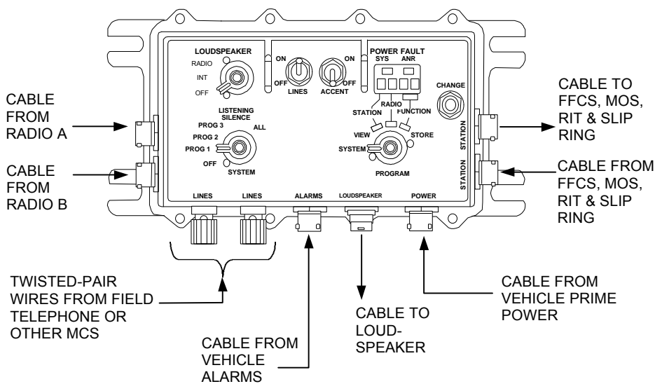
Figure 1-3. Master Control Station (MCS)
