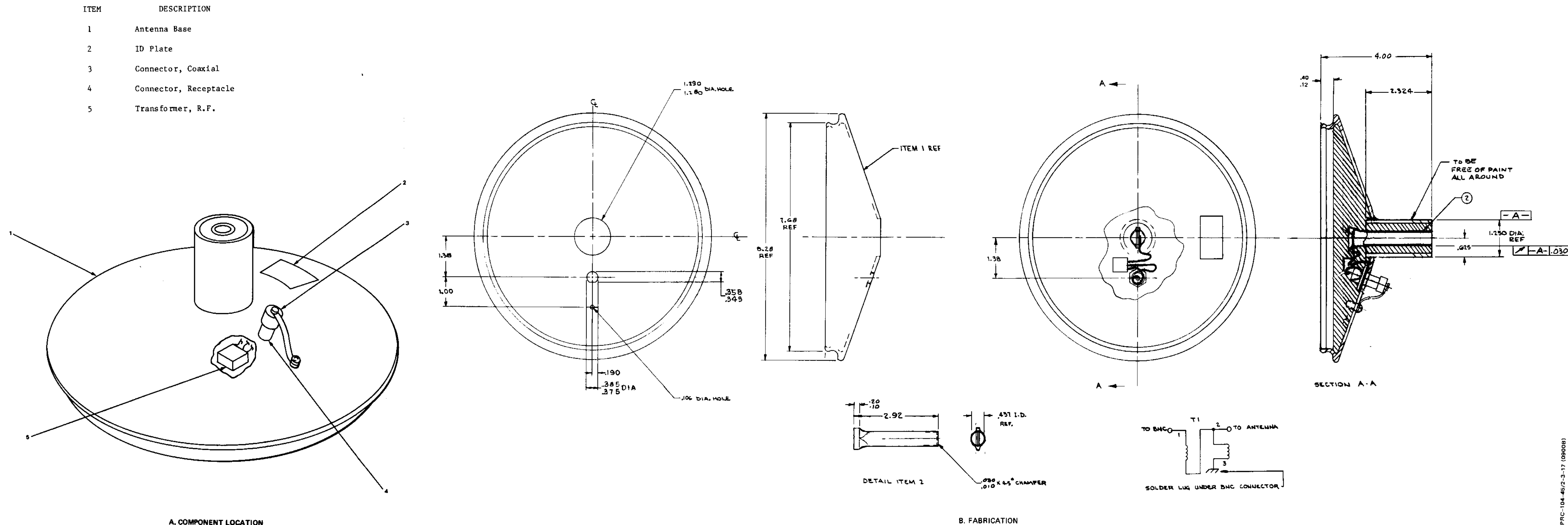
Figure 3-17. Antenna Base
