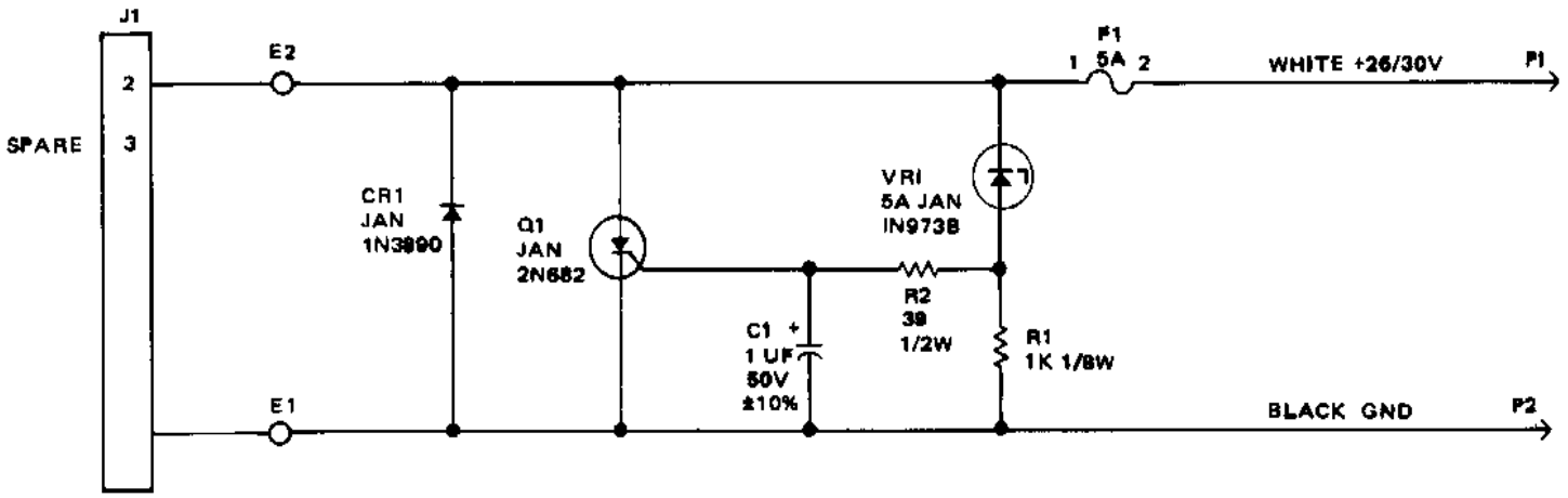
SCHEMATIC DIAGRAM
