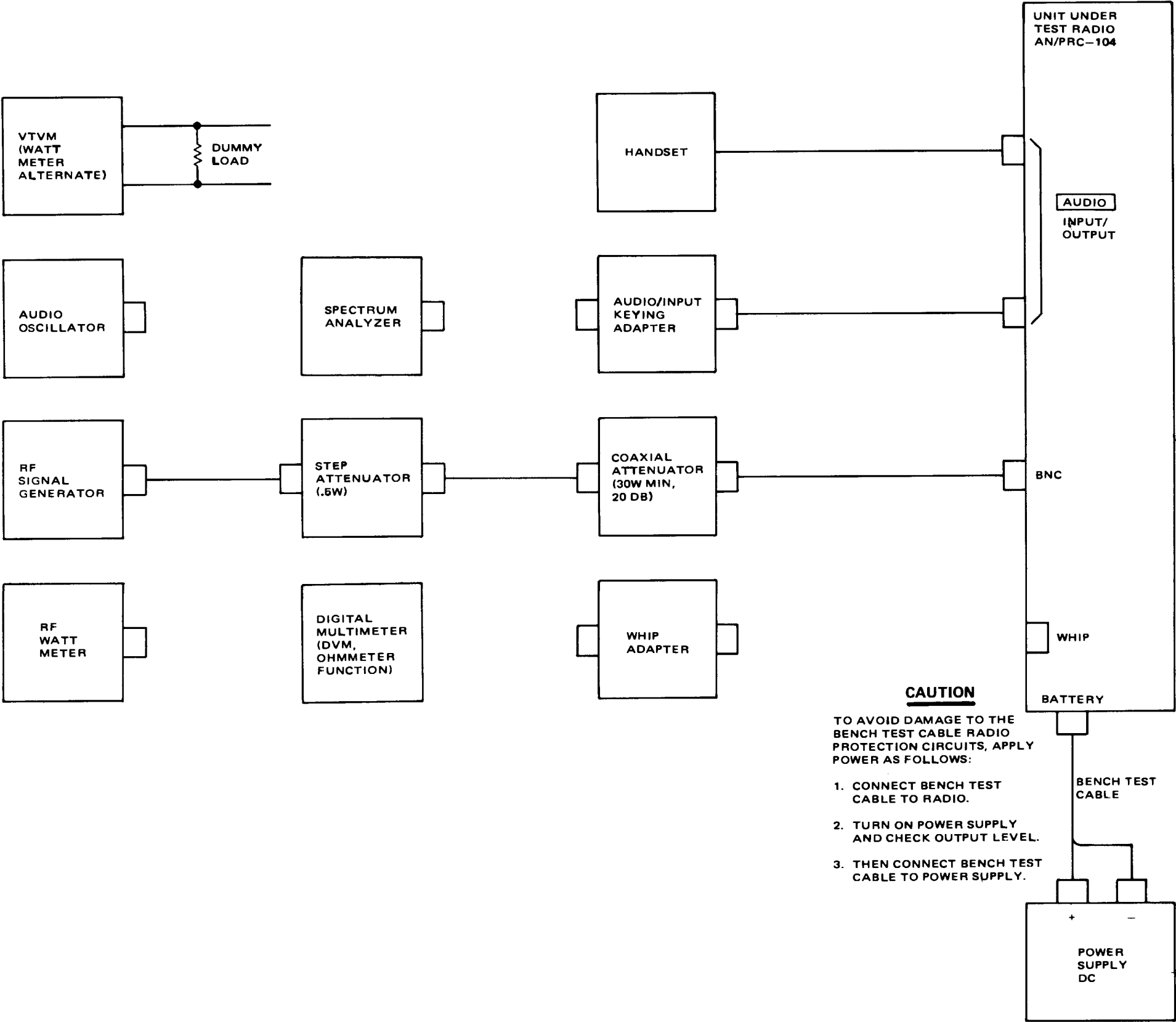
Figure 4-4. Radio Set Performance Test Setup
