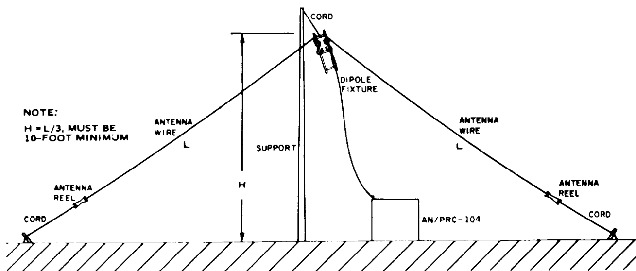
Figure A3-5. Inverted-V Dipole Antenna
