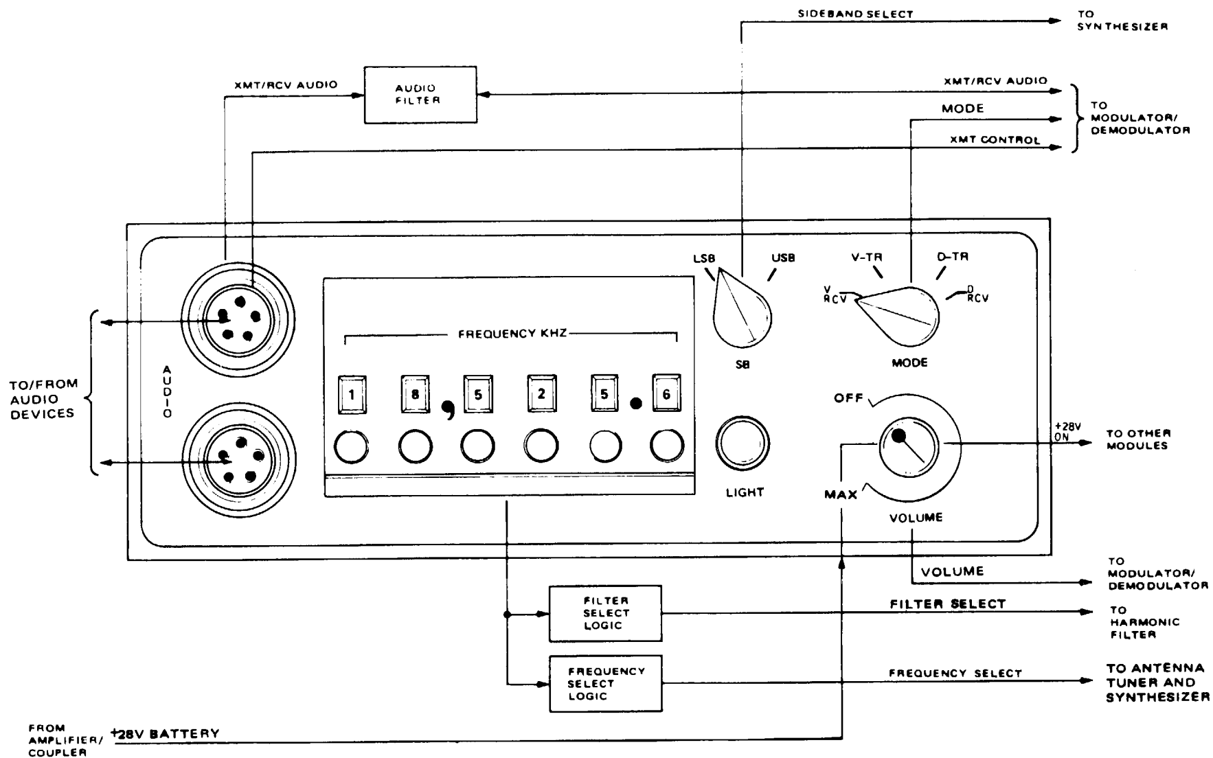
Figure 3-3. Control Panel Pictorial Block Diagram
