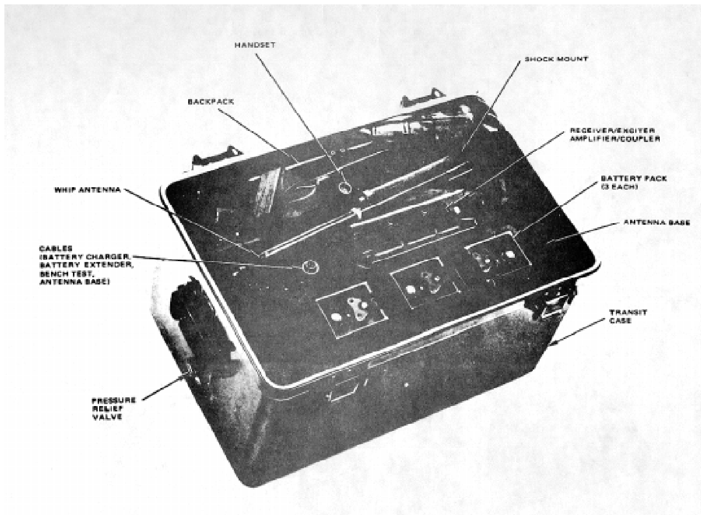
Figure 1-1. Radio Set AN/PRC-104 Equipment Supplied (Sheet 1 of 2)
