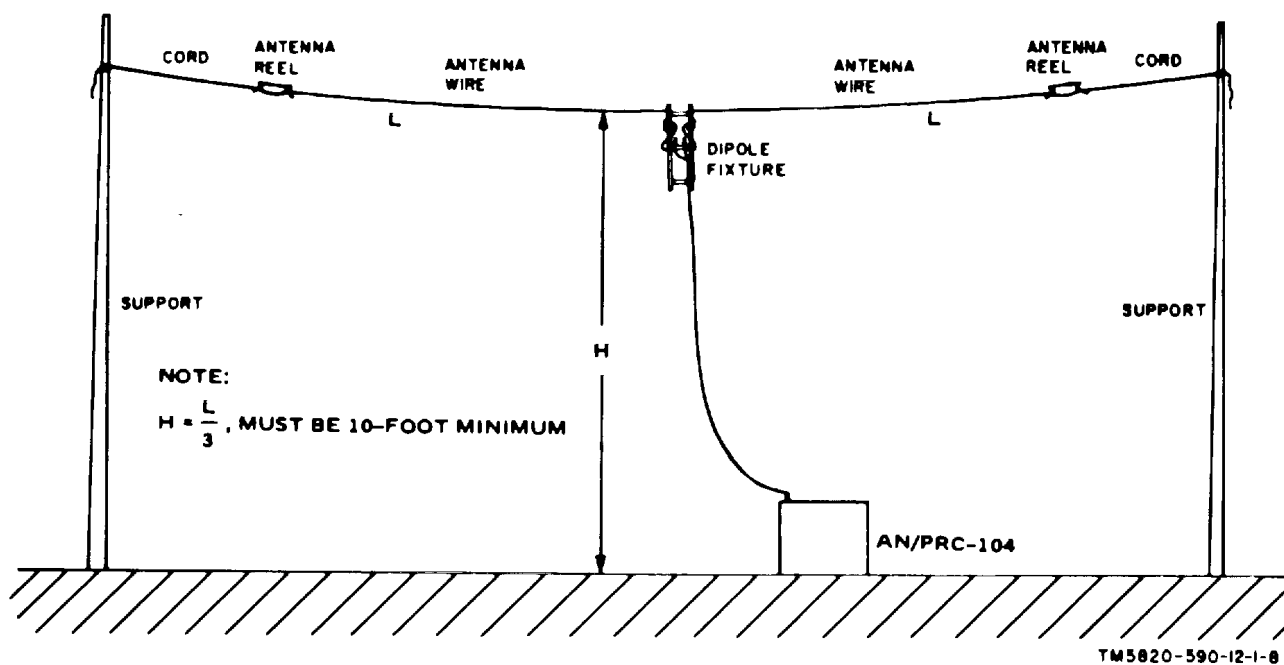
Figure A3-3. Two-Support Dipole Antenna
