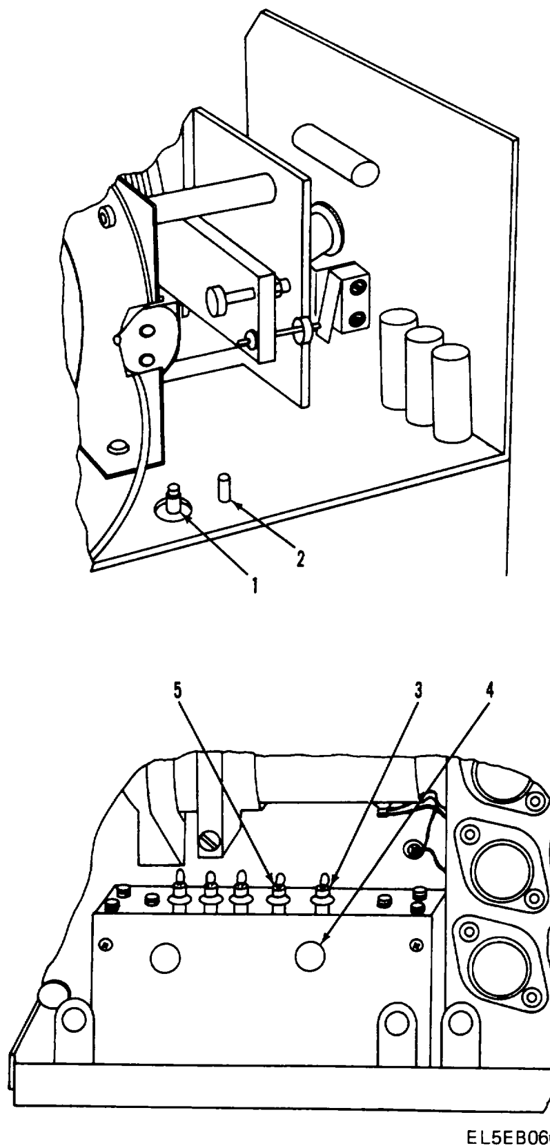
Figure 4-21 Connection and Adjustment Points - Phase Detector Adjustment
