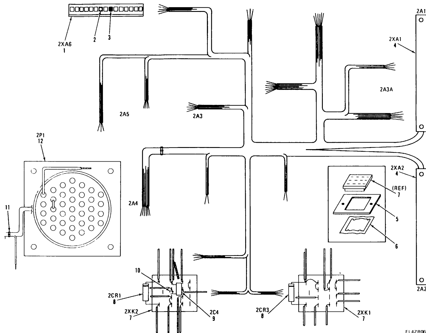
4-55 Main Harness
