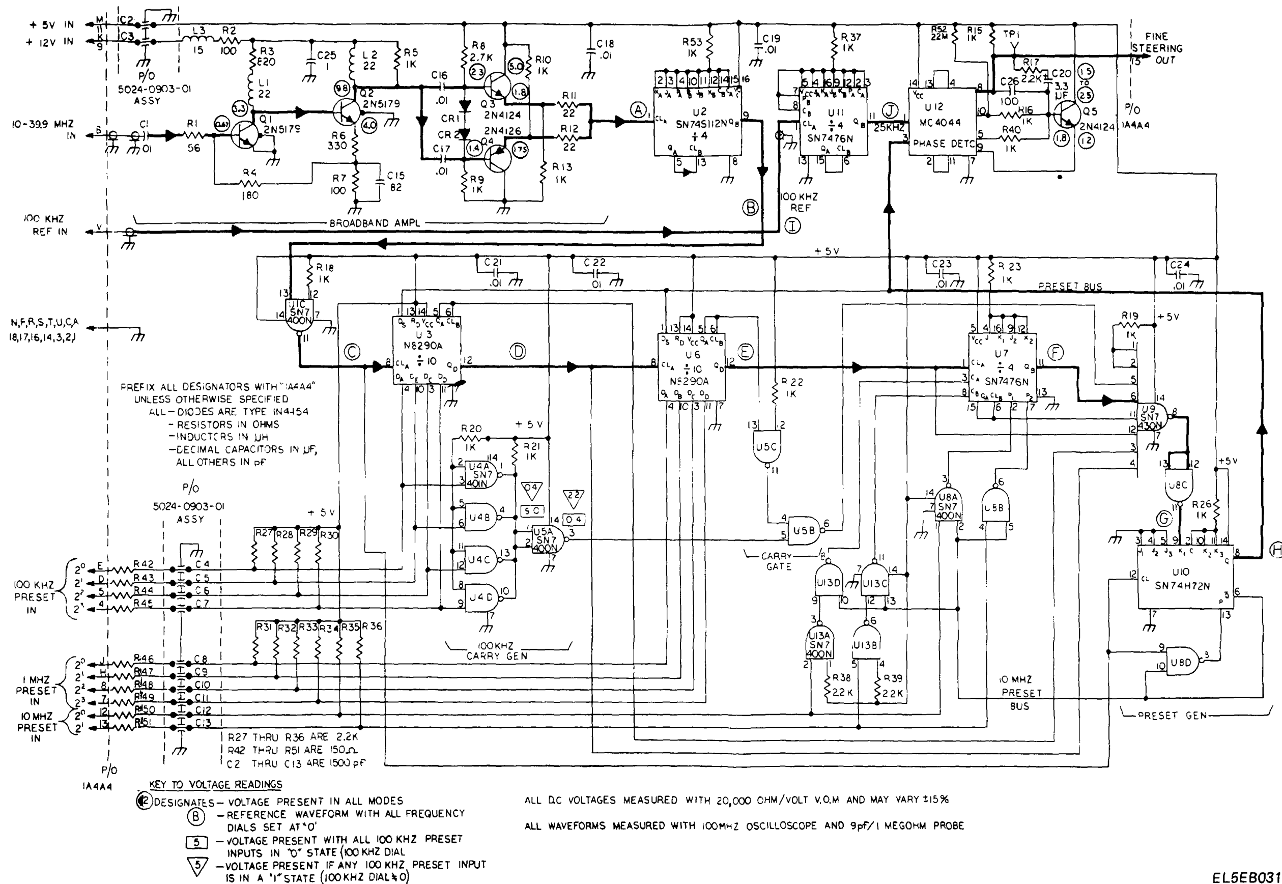
FO-21 VHF Divider Schematic
