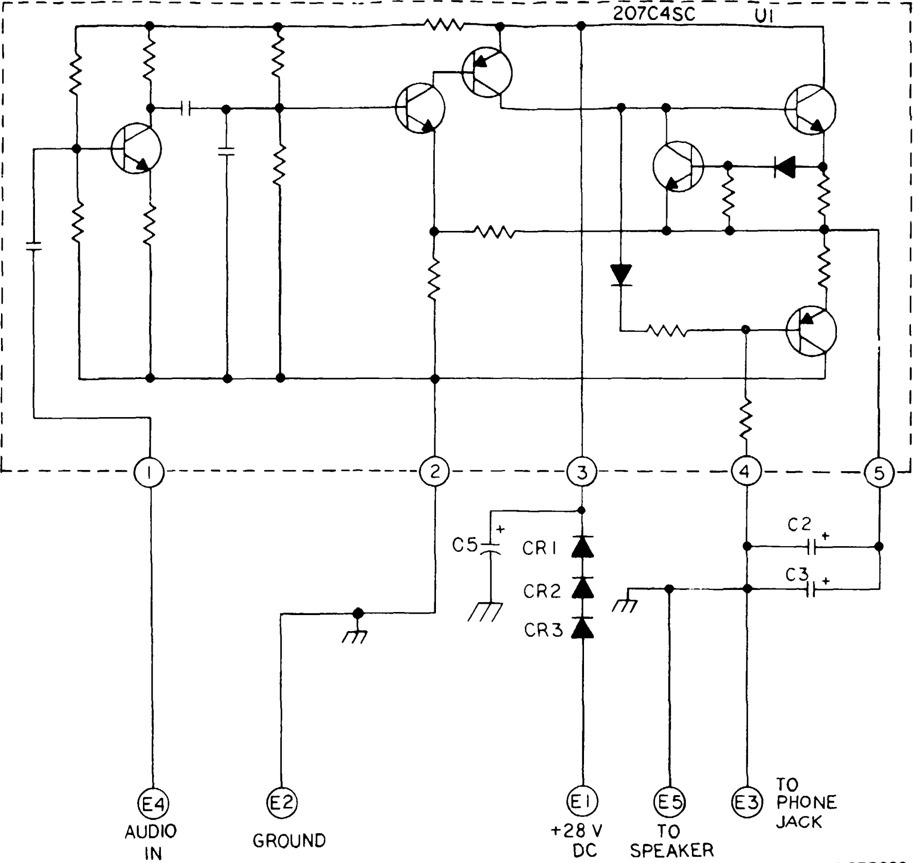
FO-12. Speaker Driver Schematic
