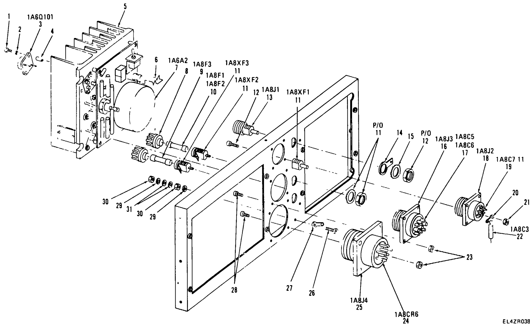
4-22 Back-Panel-Exploded View
