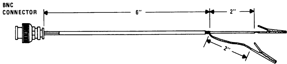
Figure 4-1. BNC/Clip Lead Cable
