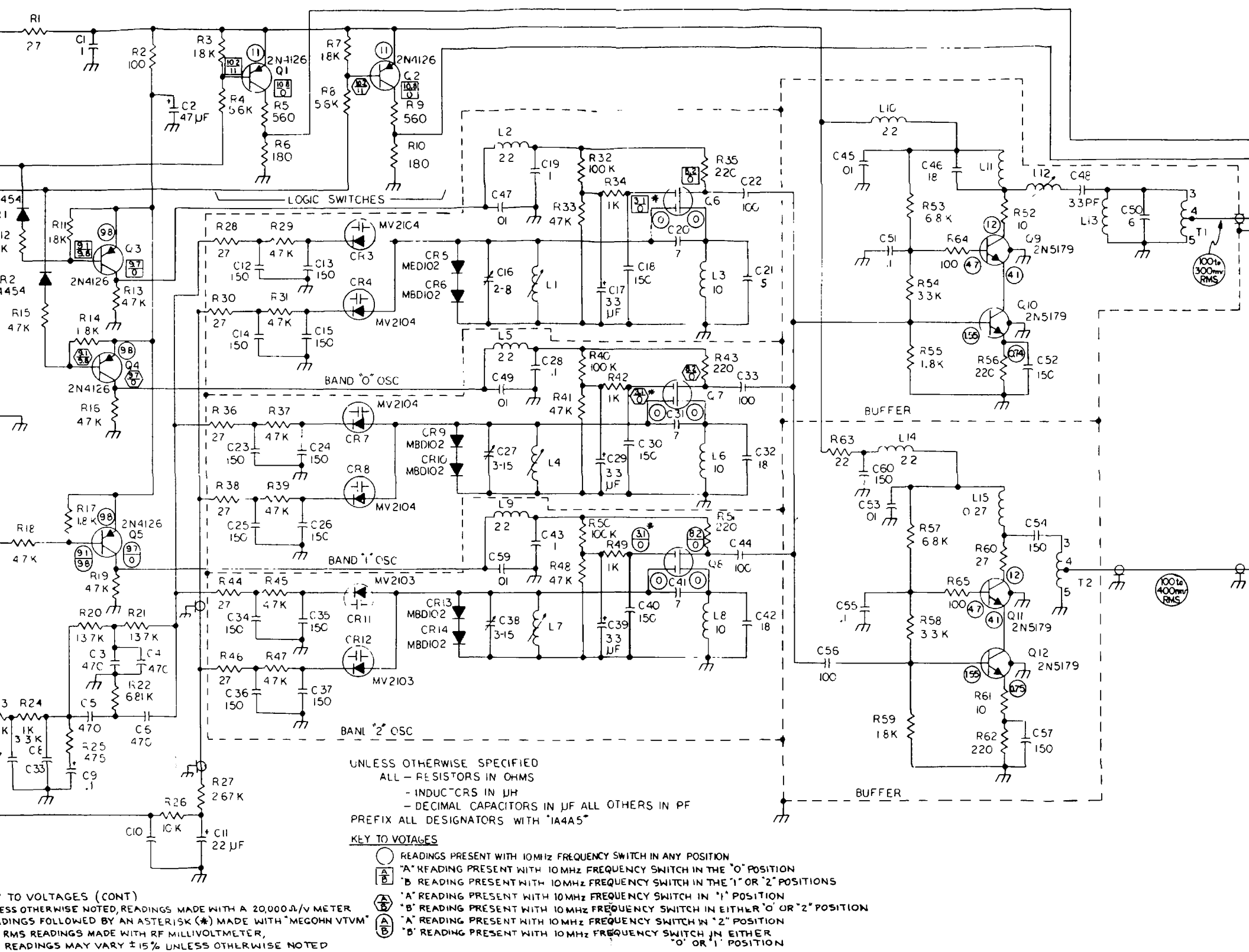
FO-22 VCO Schematic
