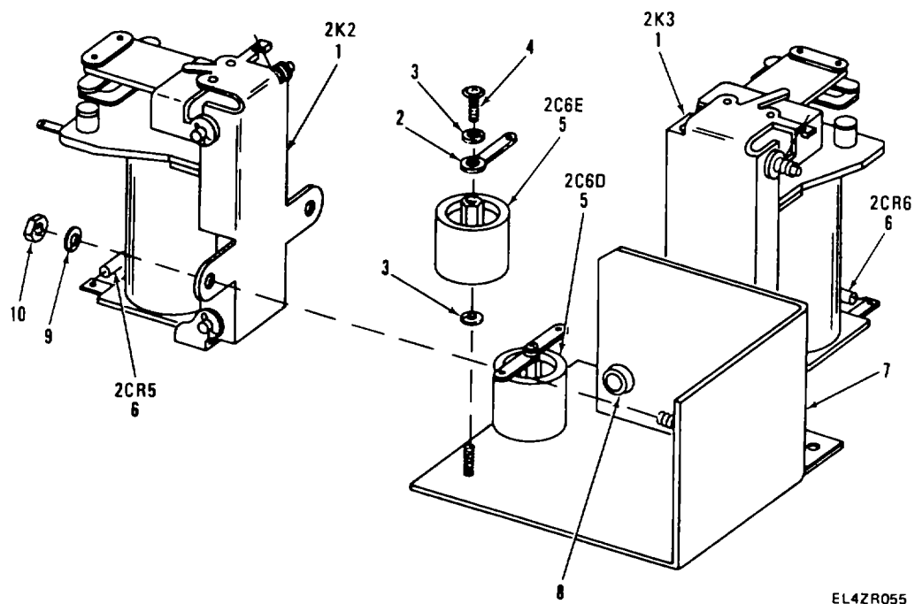
4-56 K2-K3 Relay Assembly
