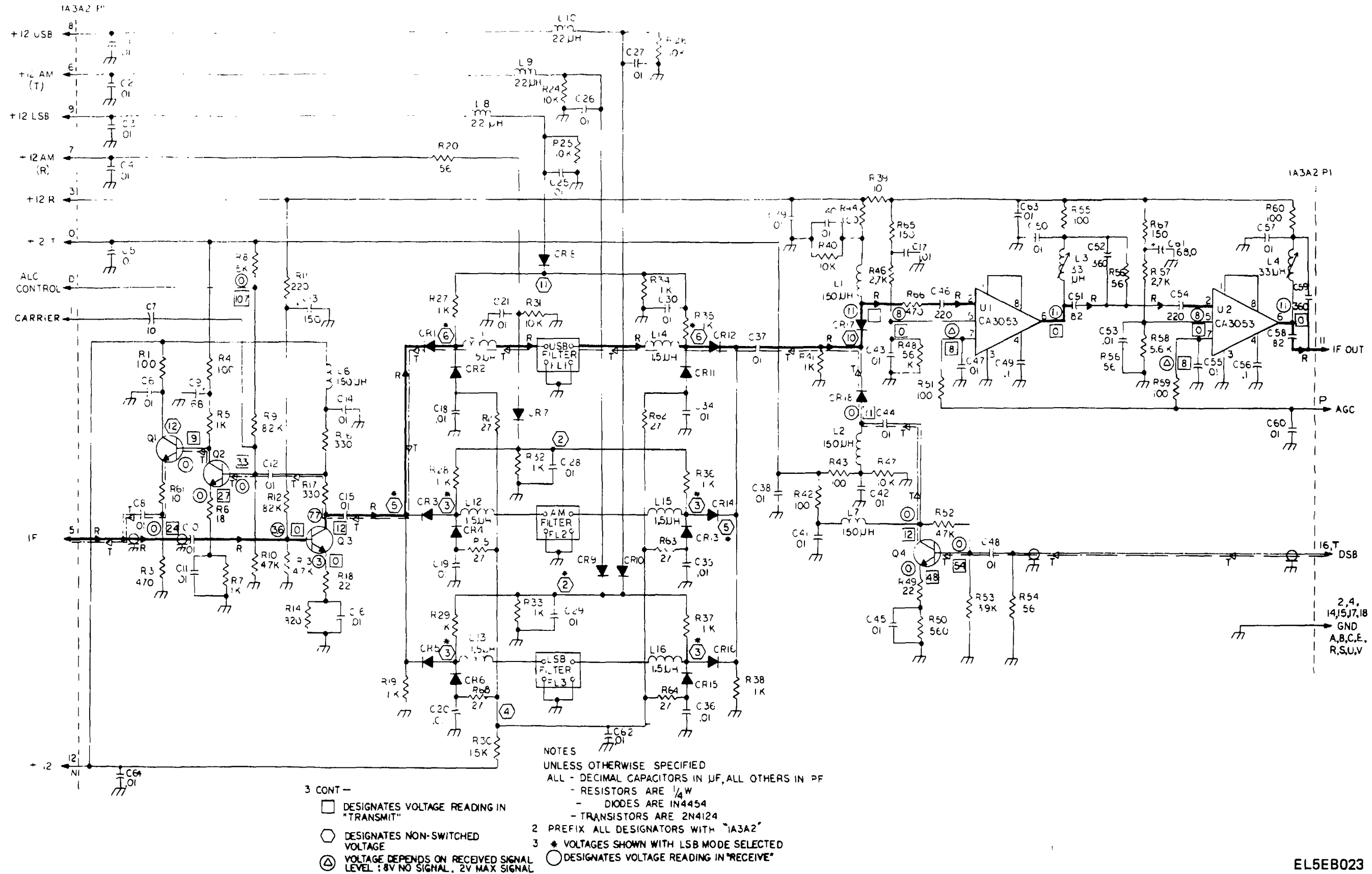
FO-15. IF Filter Schematic
