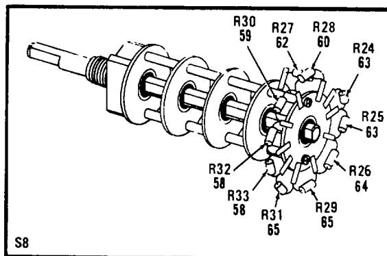
4-47 Front Panel Assembly (2 of 3)
