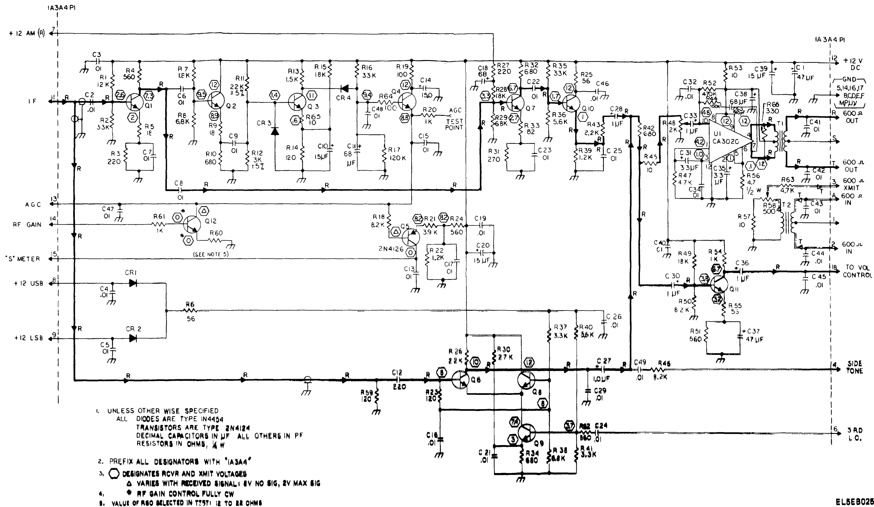
FO-17 Audio Board Schematic
