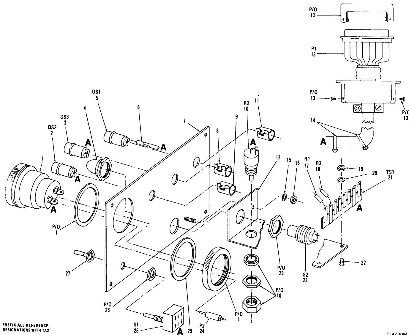
4-52 Tuning Control
