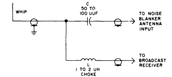
Figure 6-1. Suggested connections for using broadcast whip for both broadcast receiver and noise blanker.
