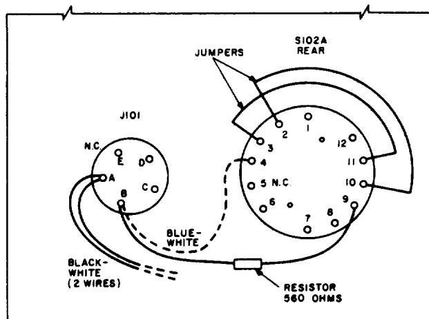
B. S102A (REAR), WIRING AFTER MODIFICATION WHEN BLUE-WHITE WIRE IS CONNECTED TO TERMINAL 4.
