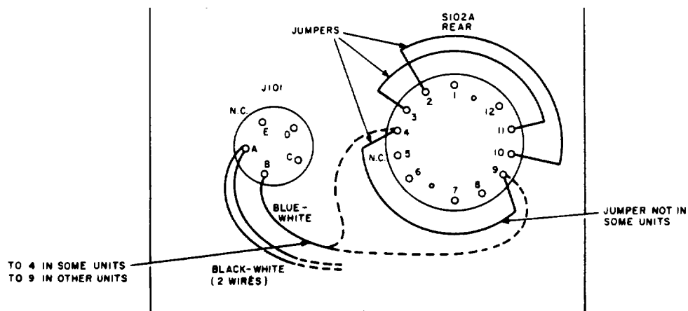
A. S102A (REAR), WIRING BEFORE MODIFICATION.
