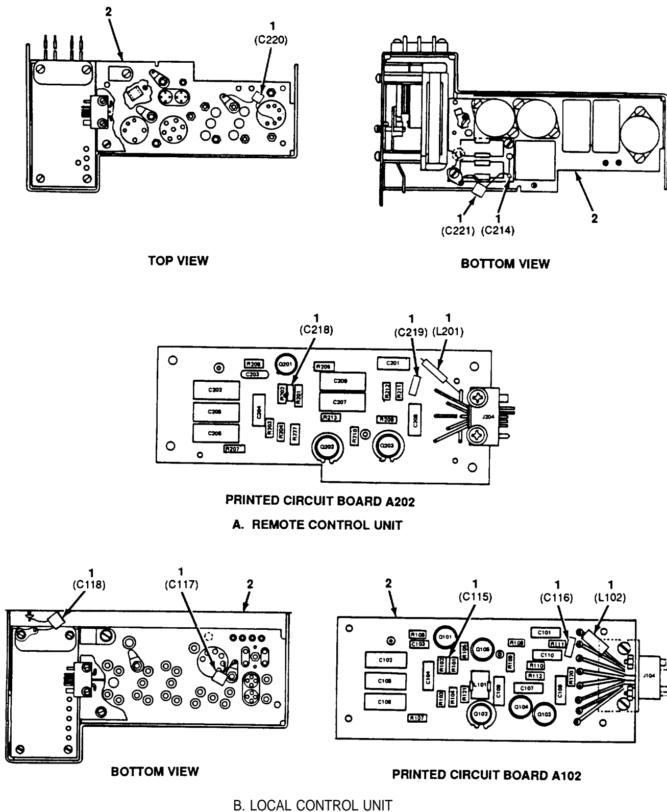
4859-008 Figure 2-7. RF Filter Assembly Components, C-2328C/GRA-39 and C-2329C/GRA-39.
