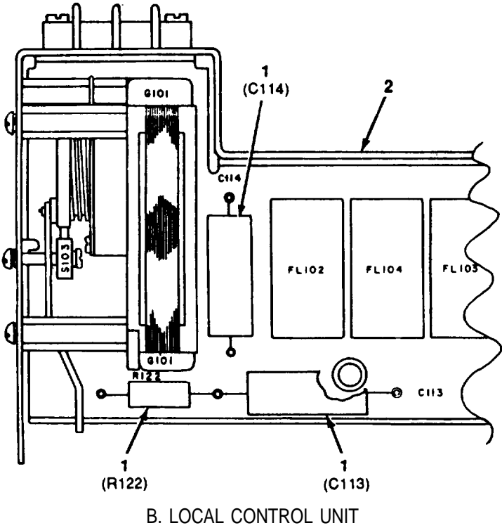
Figure 2-6. RF Filter Assembly Components, C-2328BIGRA-39 and C-2329BIGRA-39.
