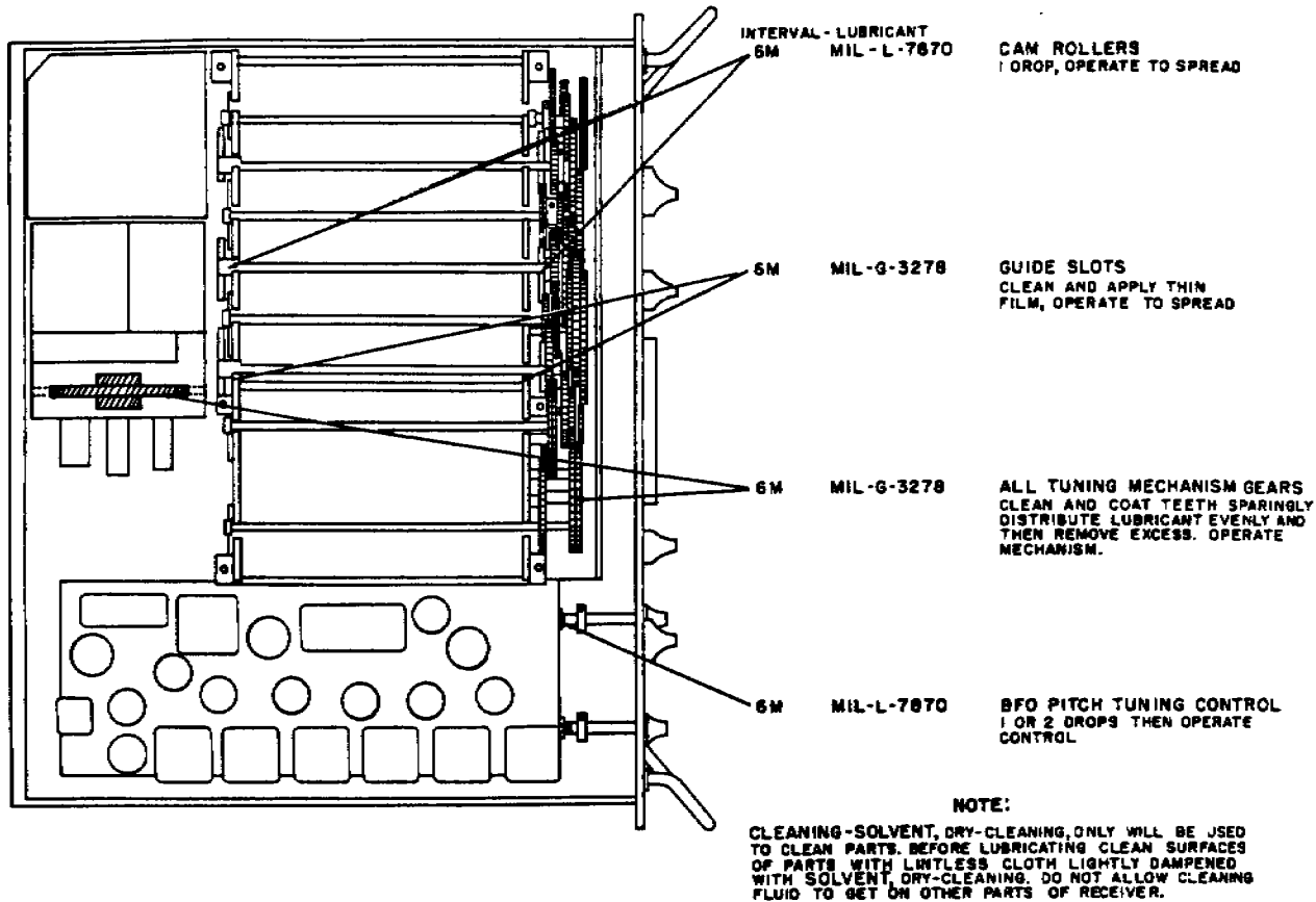
Figure 7. Lubrication.
