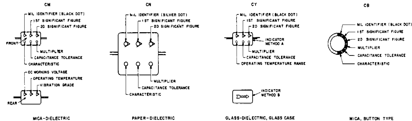
MICA-DIELECTRIC
