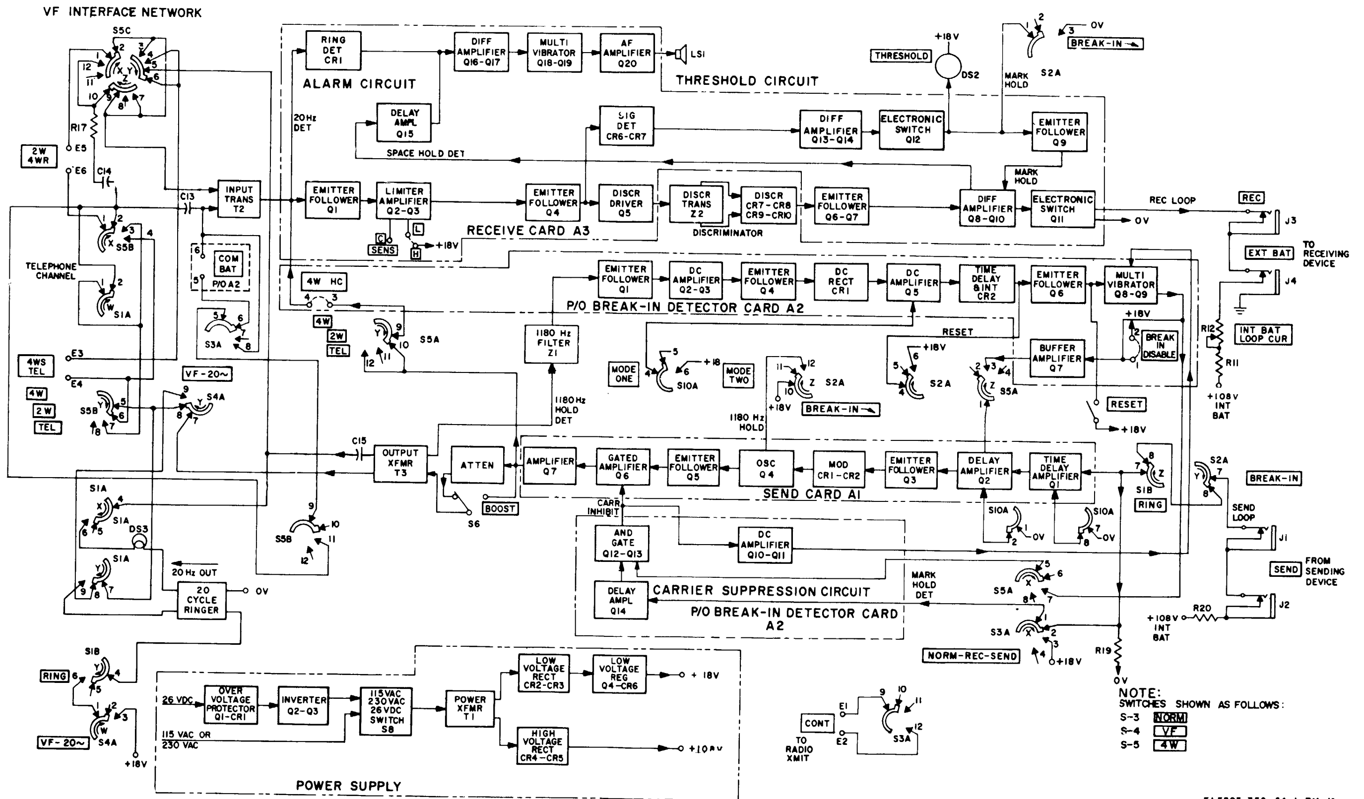
Figure FO-2. Terminal, Telegraph TH-22/TG, detailed block diagram.
