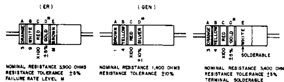
COMPOSITION-TYPE RESISTORS
