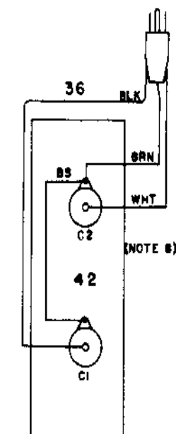
Figure FO-41(2). Terminal, Telegraph TH-22/TG, wiring diagram (sheet 2 of 2).
