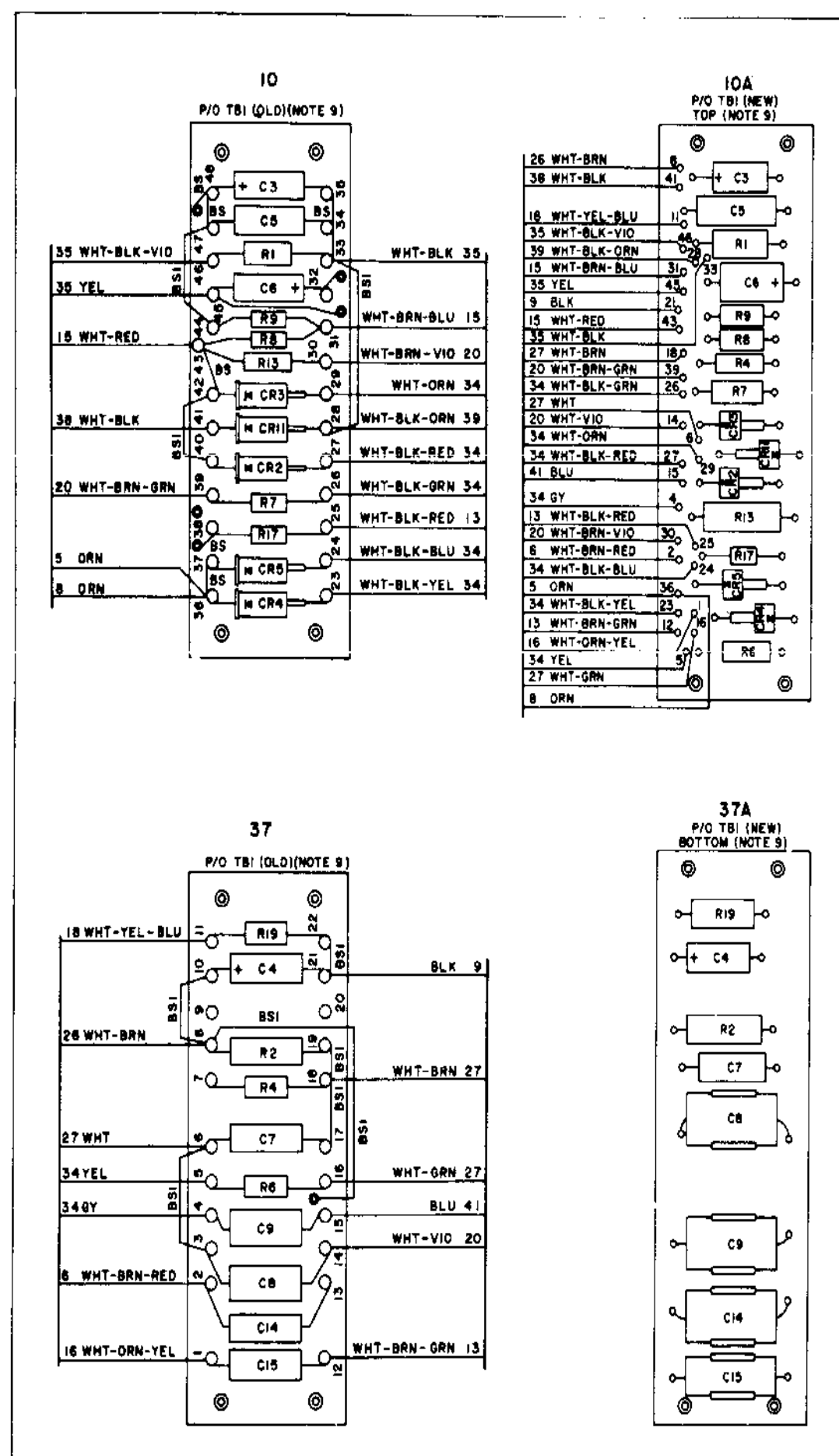
Figure FO-41(2). Terminal, Telegraph TH-22/TG, wiring diagram (sheet 2 of 2).
