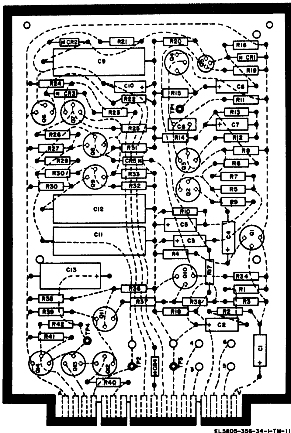
Figure 3-3. Break-in detector 1A8, component layout and wiring diagram.
