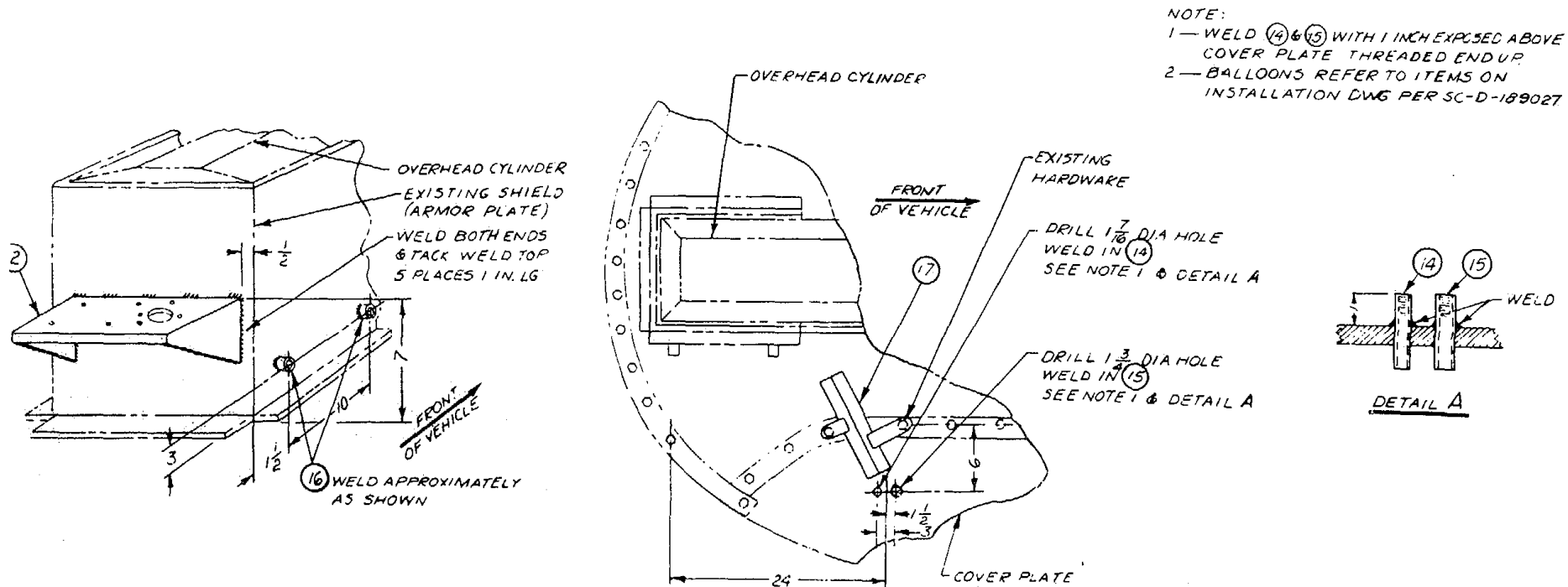
Figure 2-3. Drilling and welding.
