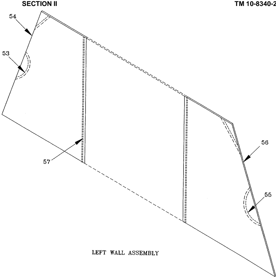
Figure 2. TENT BODY ASSEMBLY (Sheet 6 of 10)
