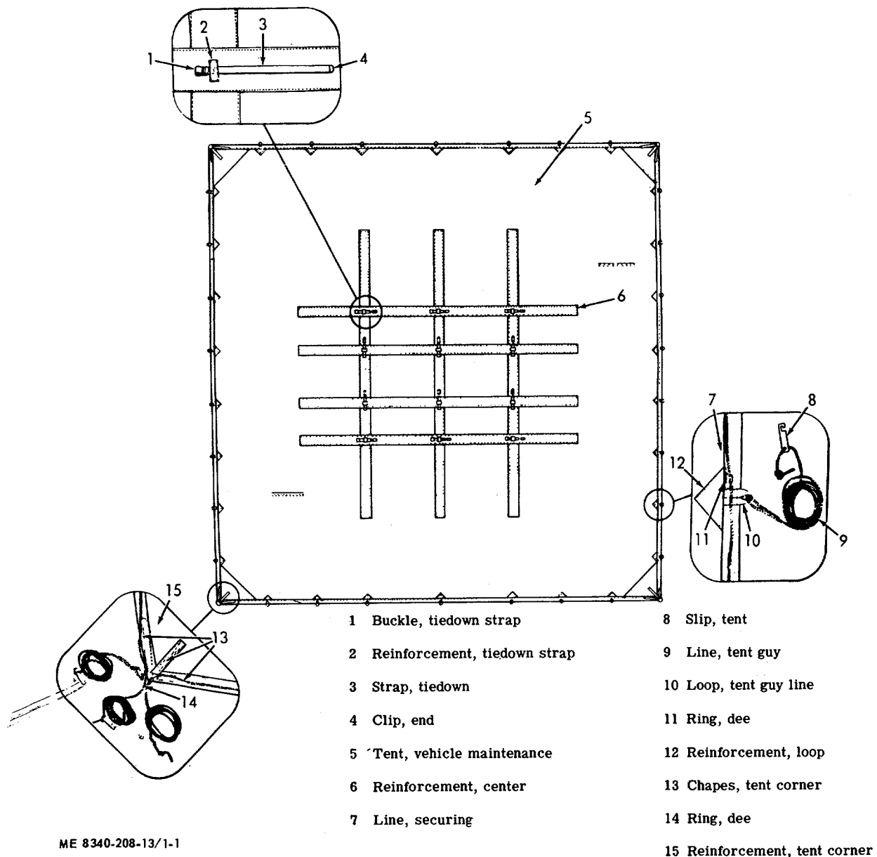
Figure 1-1. Vehicle maintenance tent
