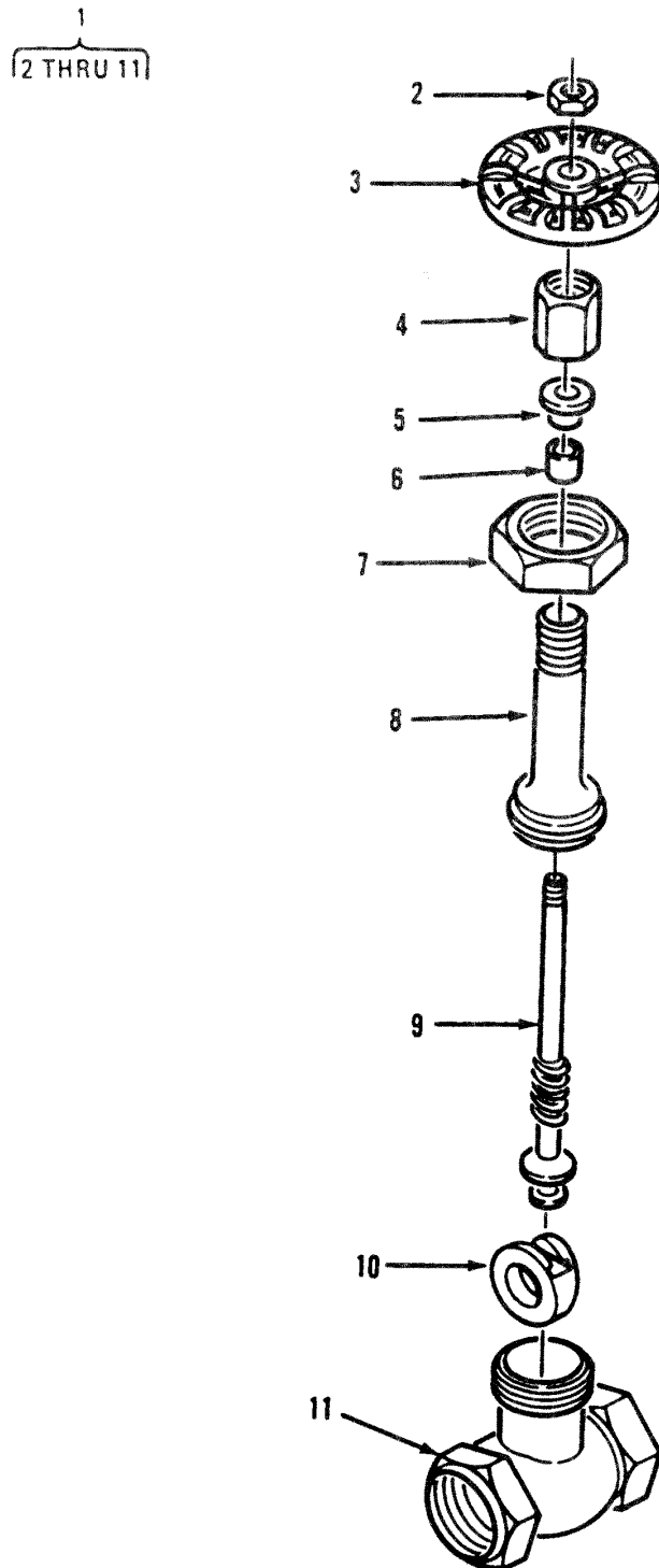
Figure 12. Tank, 2-Inch Gate Valve Assembly
