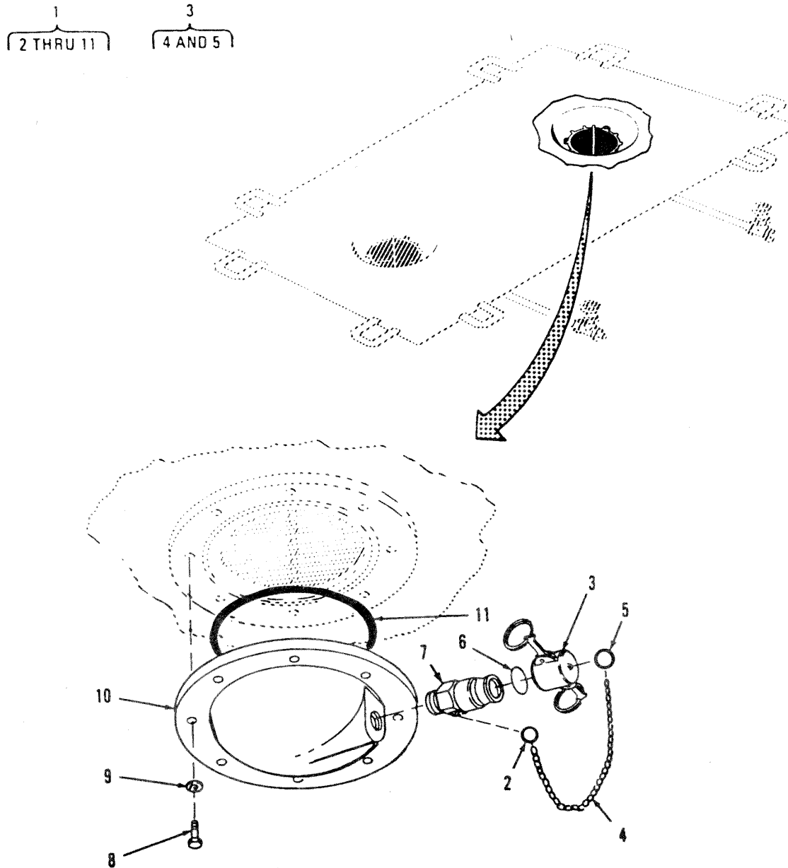
Figure 8. BERM LINER Drain Fitting Assembly
