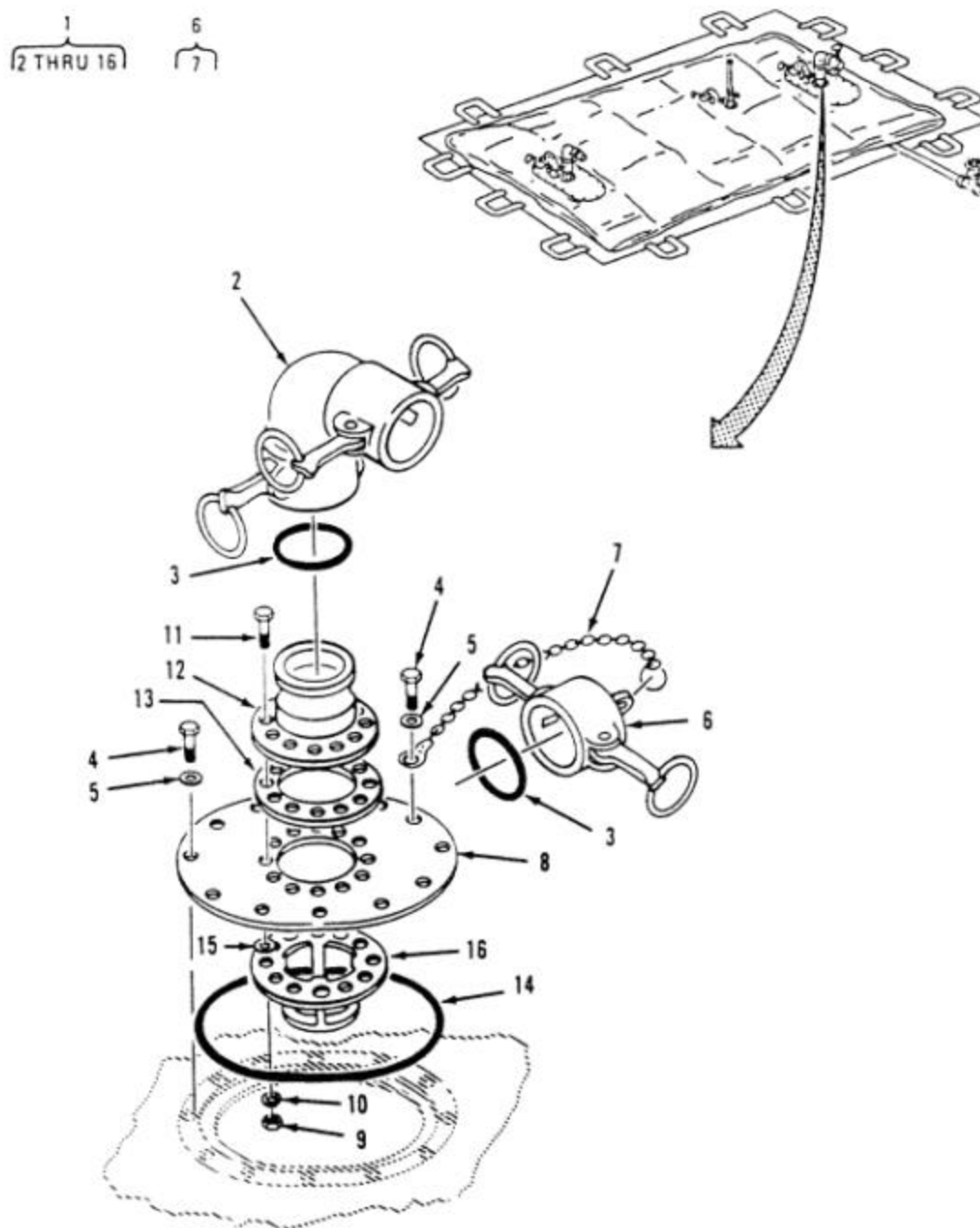
Figure 2. Tank Filler Assembly
