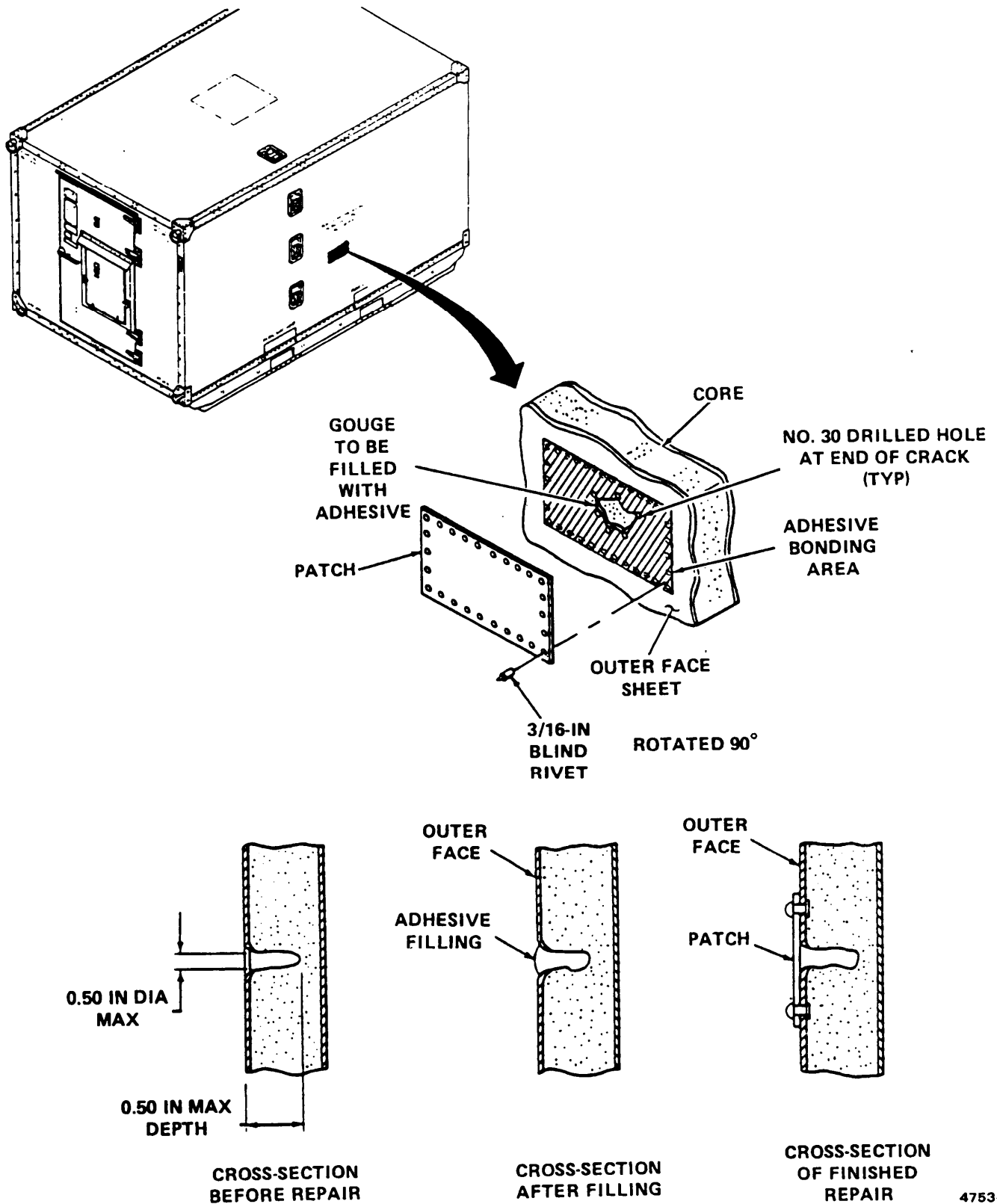
Figure 4-10. Panel Repair
