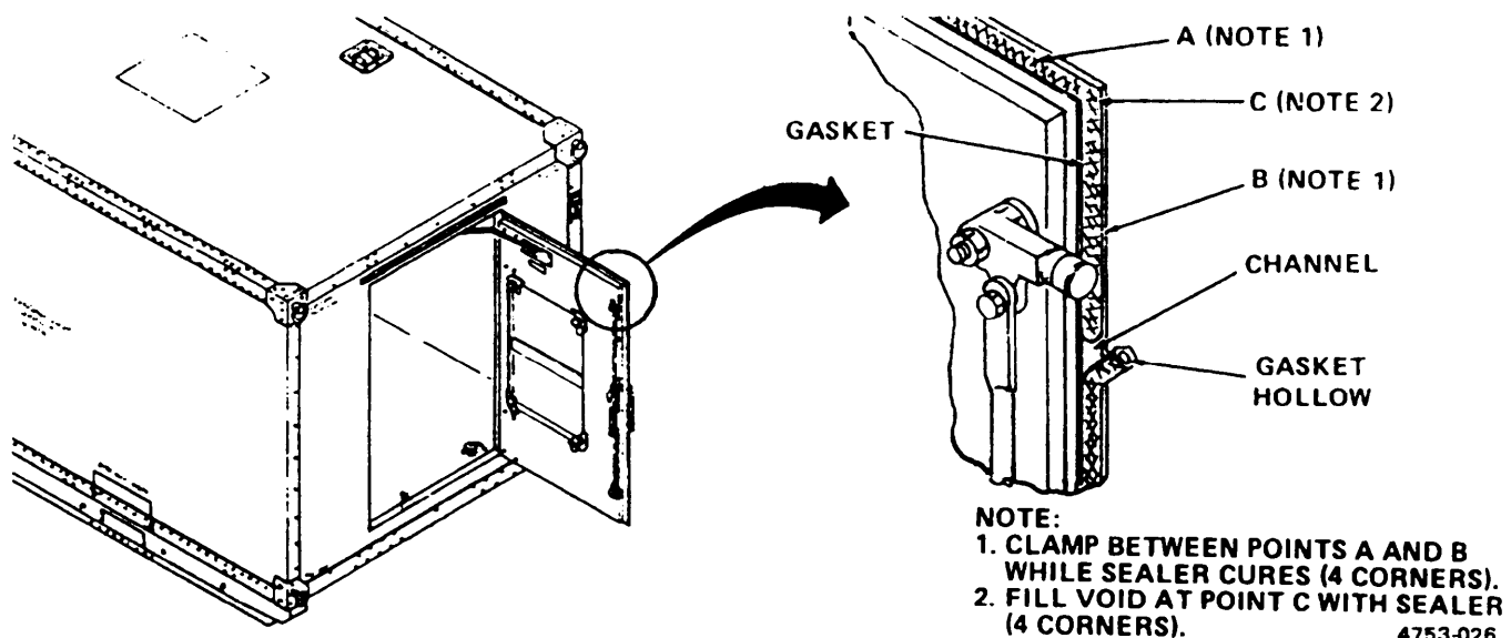
Figure 4-4. Weather Gasket Replacement.
