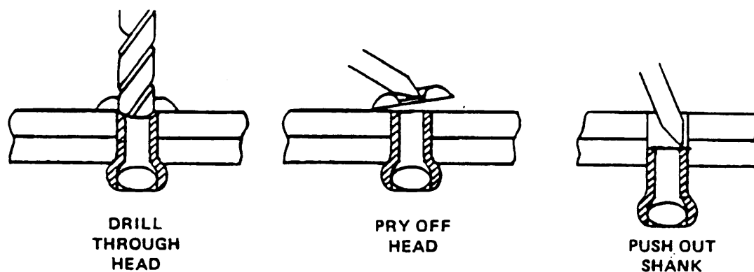
Figure 3-5. Removing Blind Rivets.
