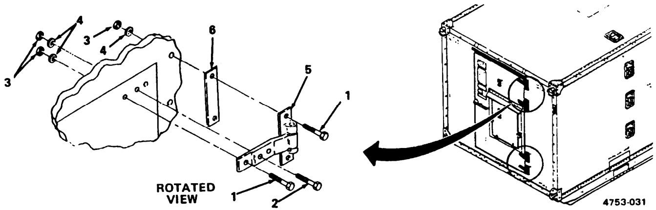
Figure 4-9. Door Hinge Assembly Replacement.
