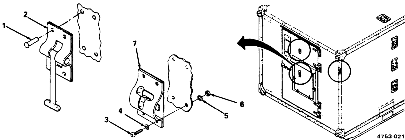
Figure 3-12. T-Latch and Holder Replacement.
