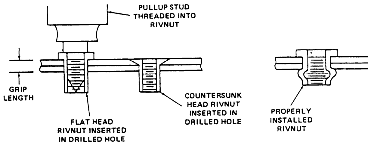
Figure 3-7. Installing Rivnuts.
