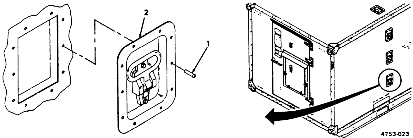
Figure 3-16. Recessed Step Pan Assembly Replacement.
