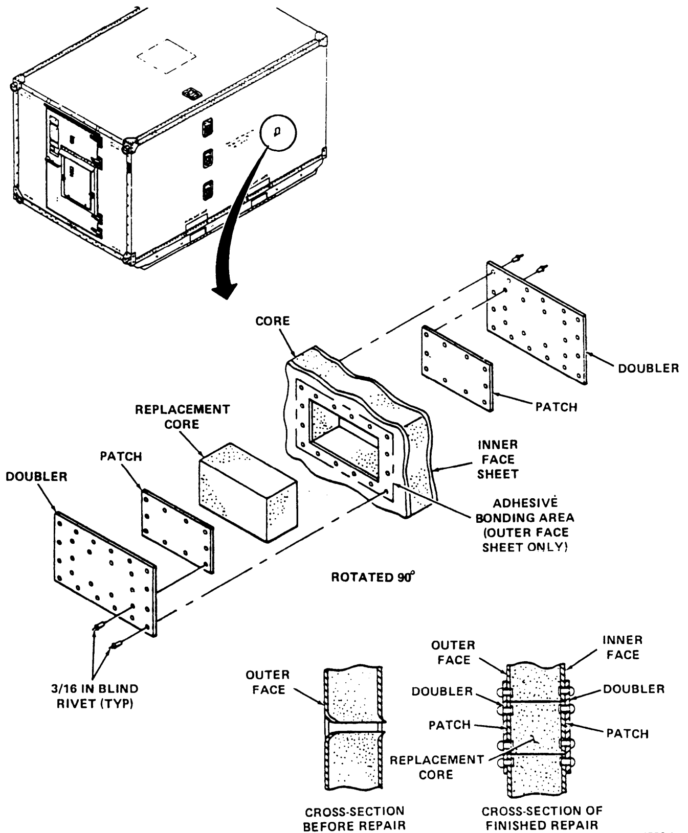
Figure 5-5. Panel Repair.
