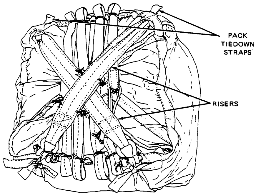
Figure 2-36. Risers Stowed and Clevis Temporarily Secured.
