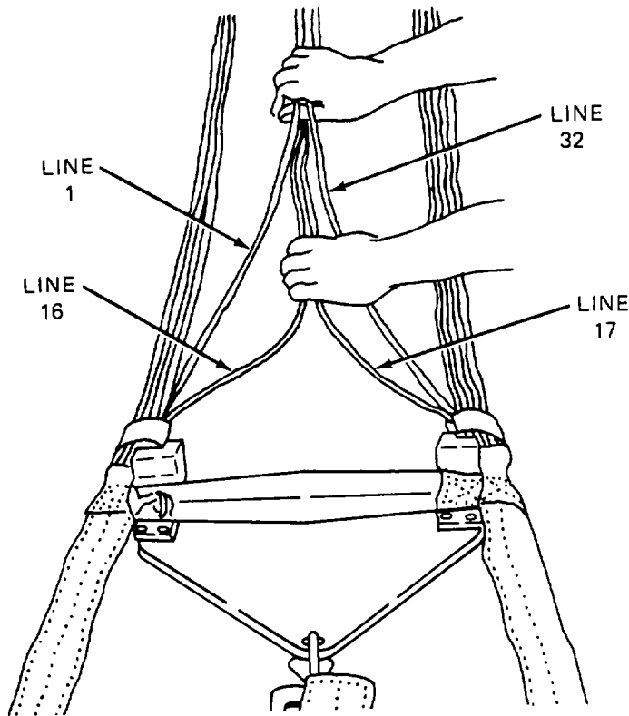
Figure 2-15. Proper Layout.
