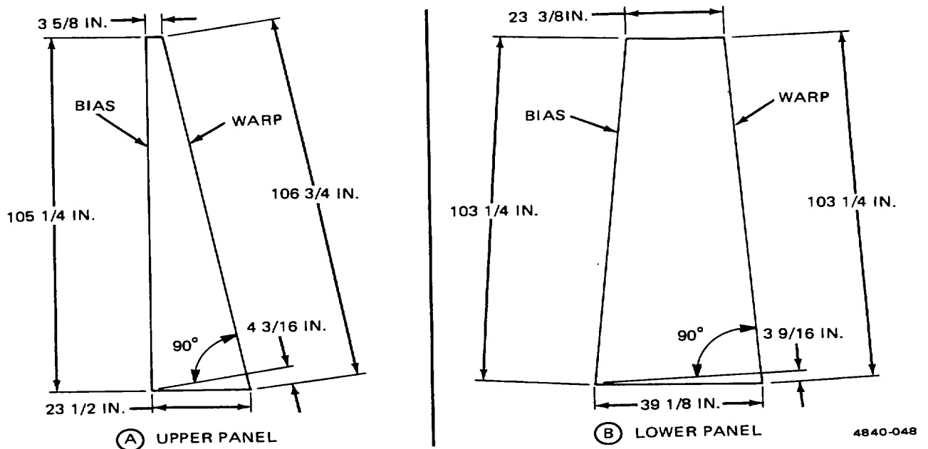
Figure 2-46. Canopy Panel Fabrication Details.
