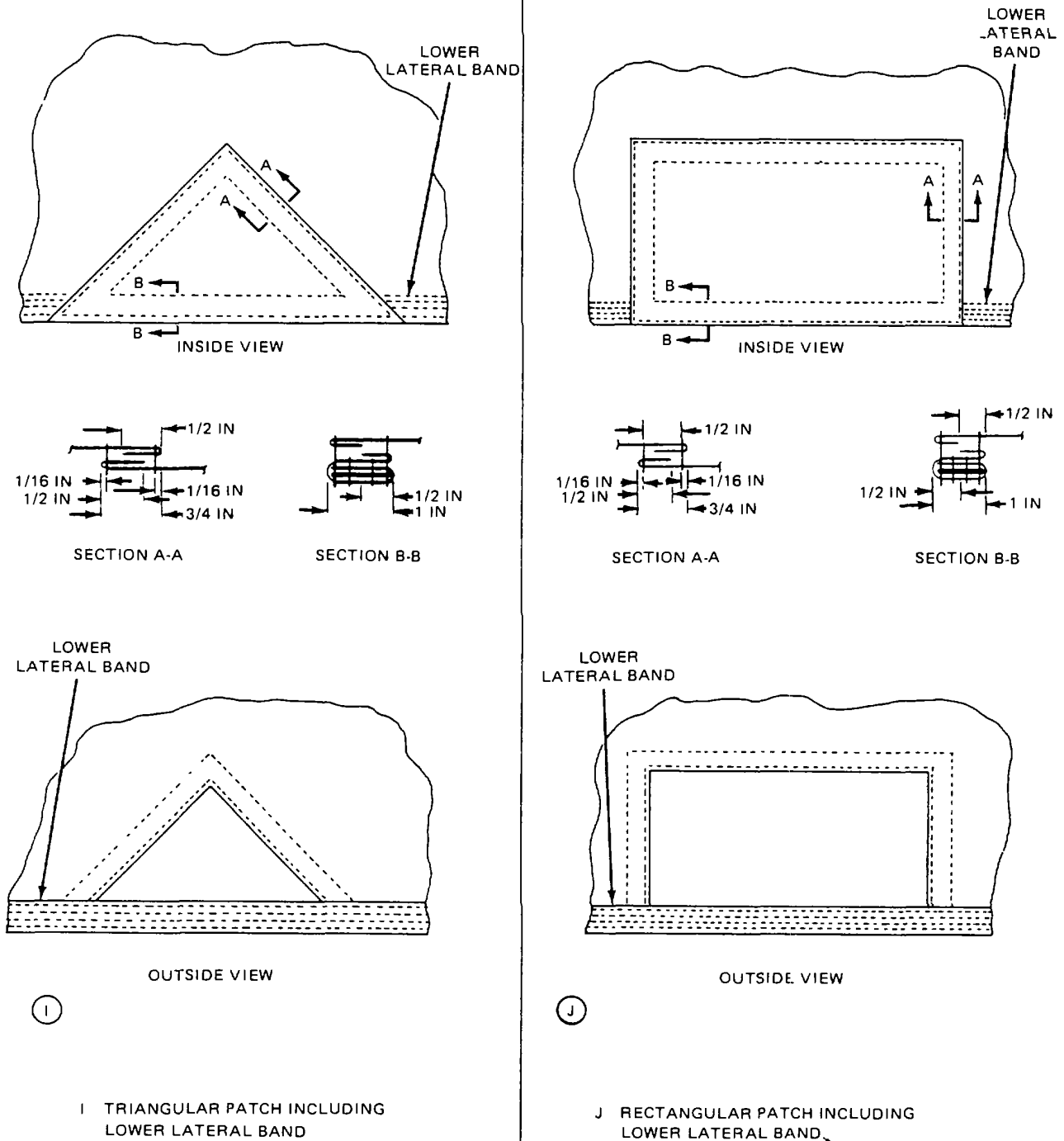
Figure 2-77. Common Miscellaneous Canopy Patches (Sheet 5 of 6).
