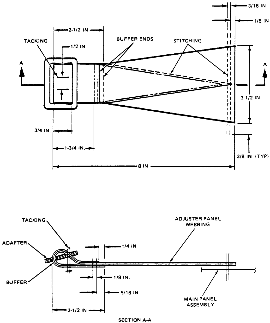
Figure 2-134. Waistband Adjuster Panel Fabrication.
