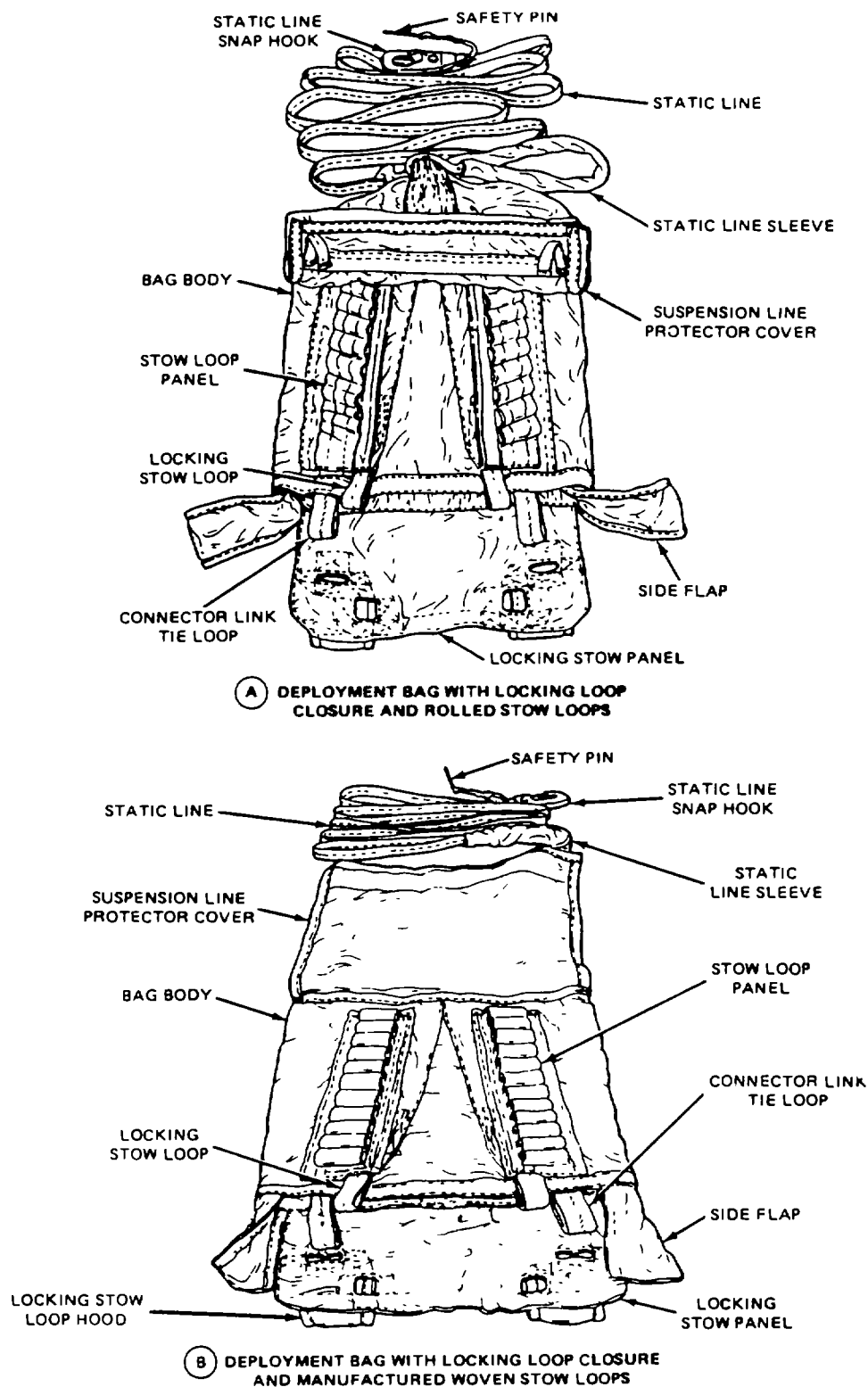
Figure 1-4. Deployment Bag.
