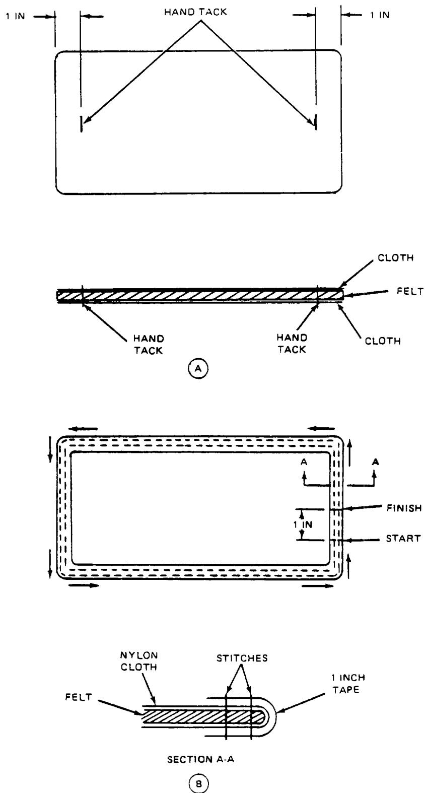
Figure 2-117. Ejector Snap Pad Construction Details.
