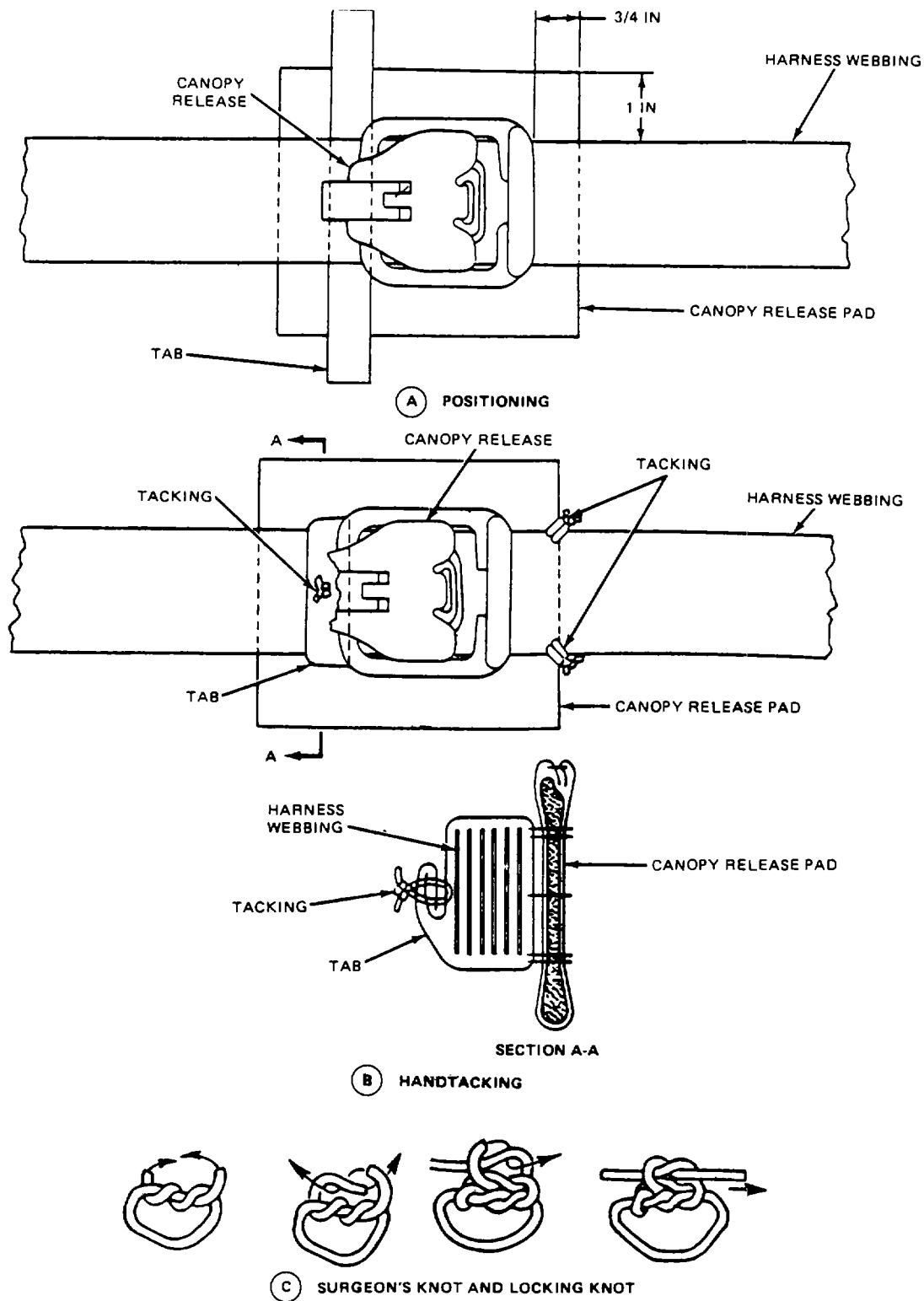
Figure 2-115. Assembly of canopy Release Pad to Harness.
