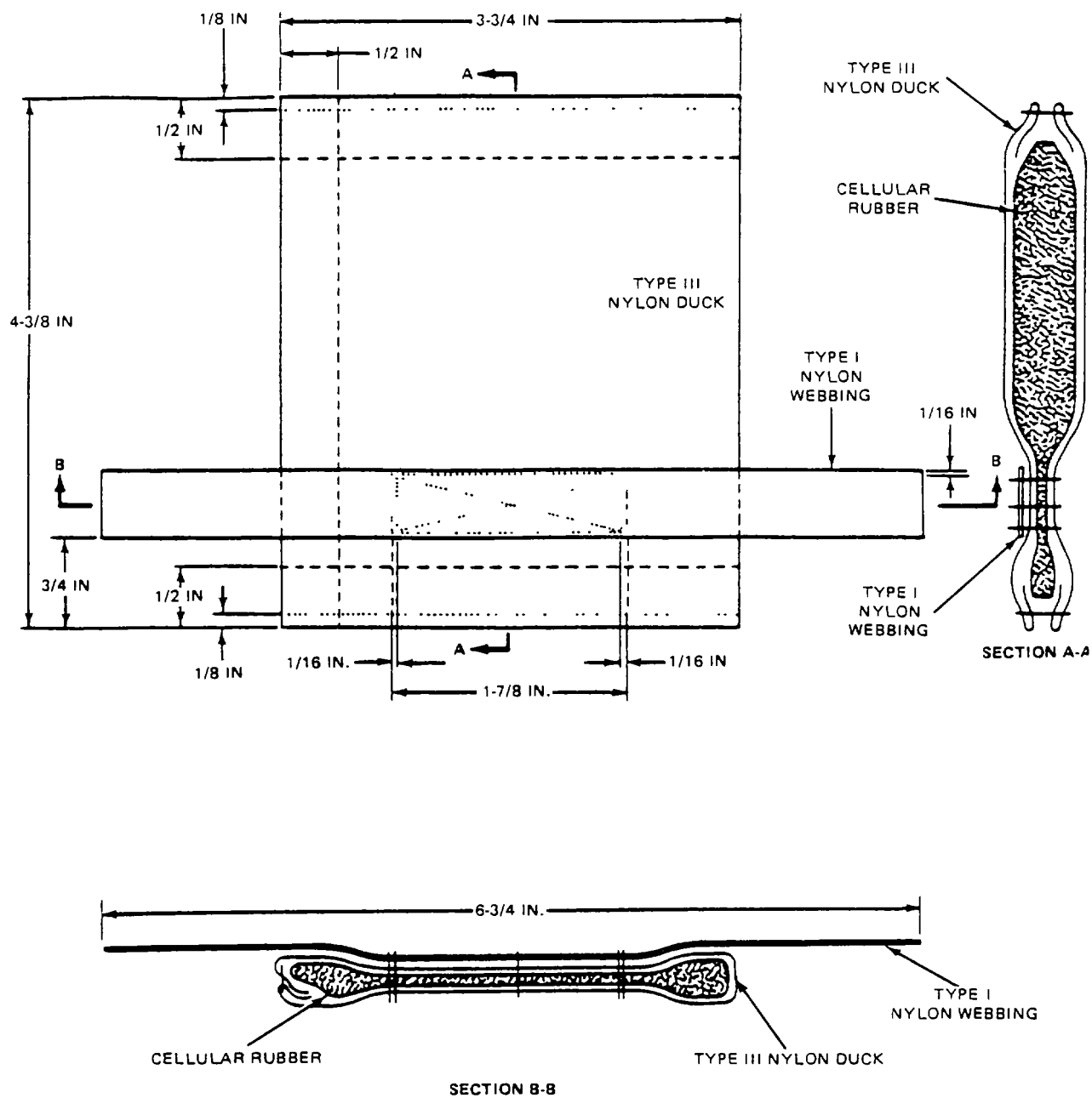
Figure 2-114. Canopy Release Pad Construction Details.
