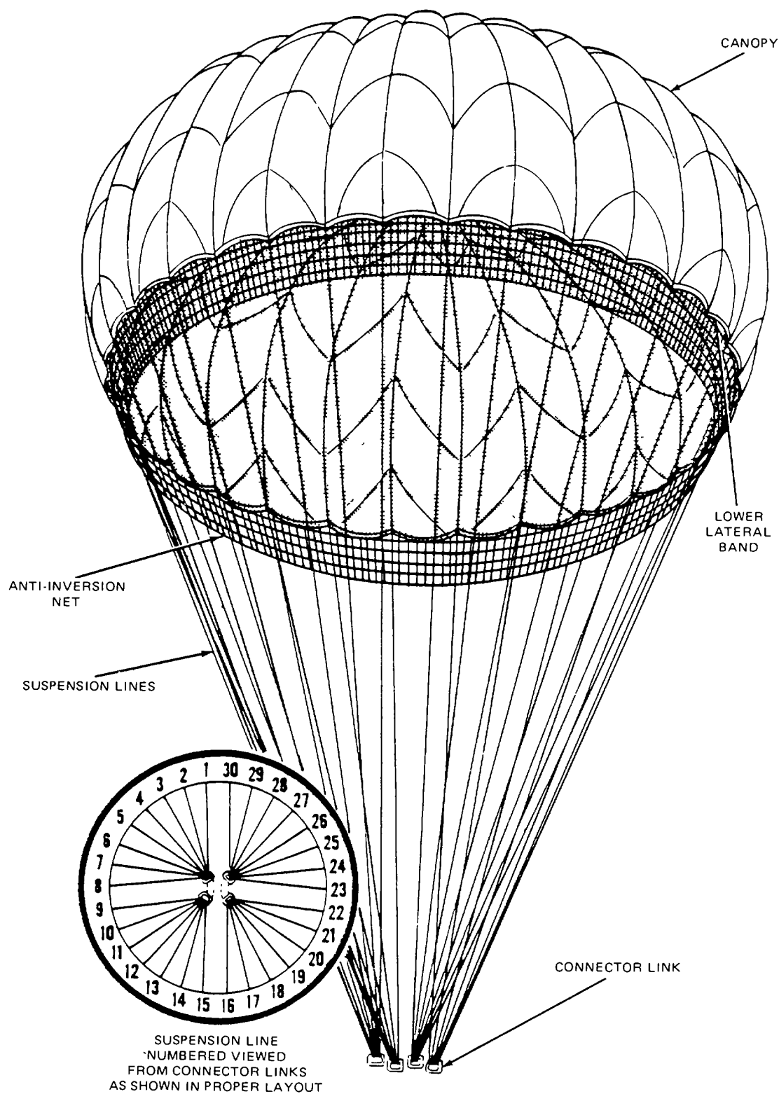
Figure 1-2. Canopy Assembly.
