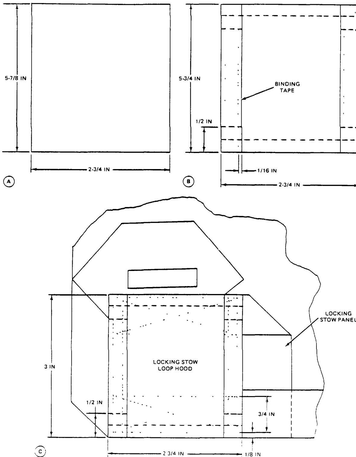
Figure 2-105. Locking Stow Loop Hood Replacement.
