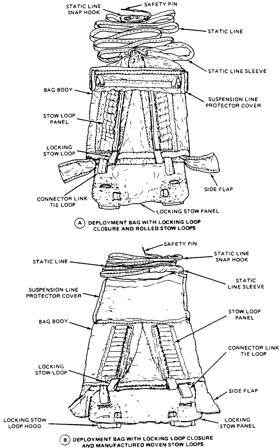
Figure 2-98. Deployment Bags with Woven and Rolled Stow Loops.
