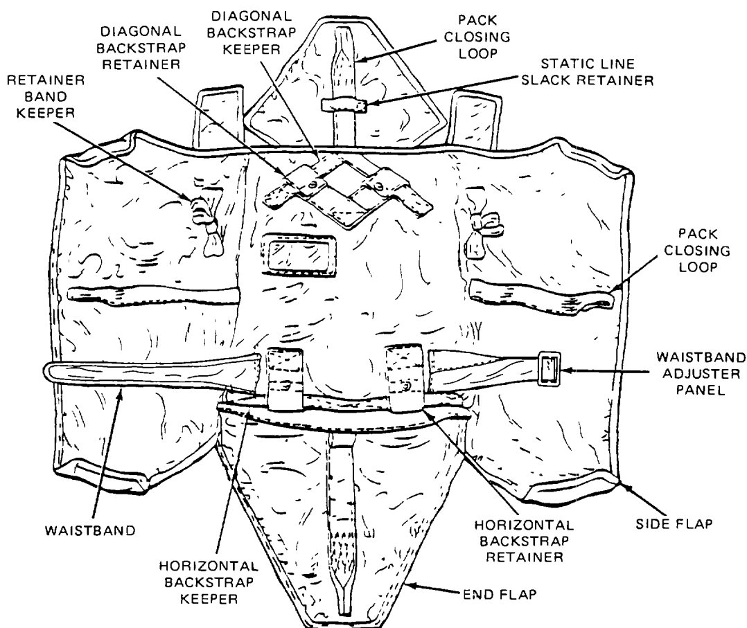
Figure 1-3. Pack Tray.
