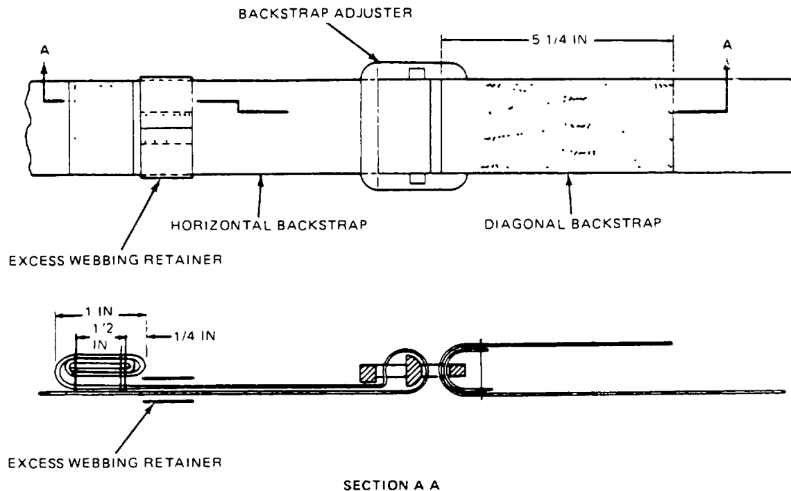
Figure 2-111. Replacement of Horizontal Back strap.
