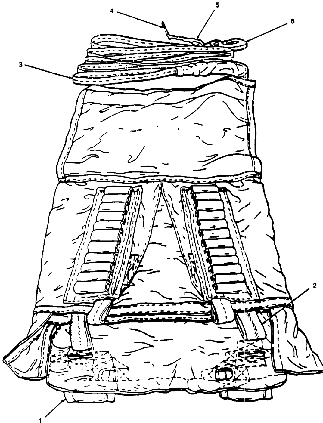
Figure C-3. Deployment Bag
