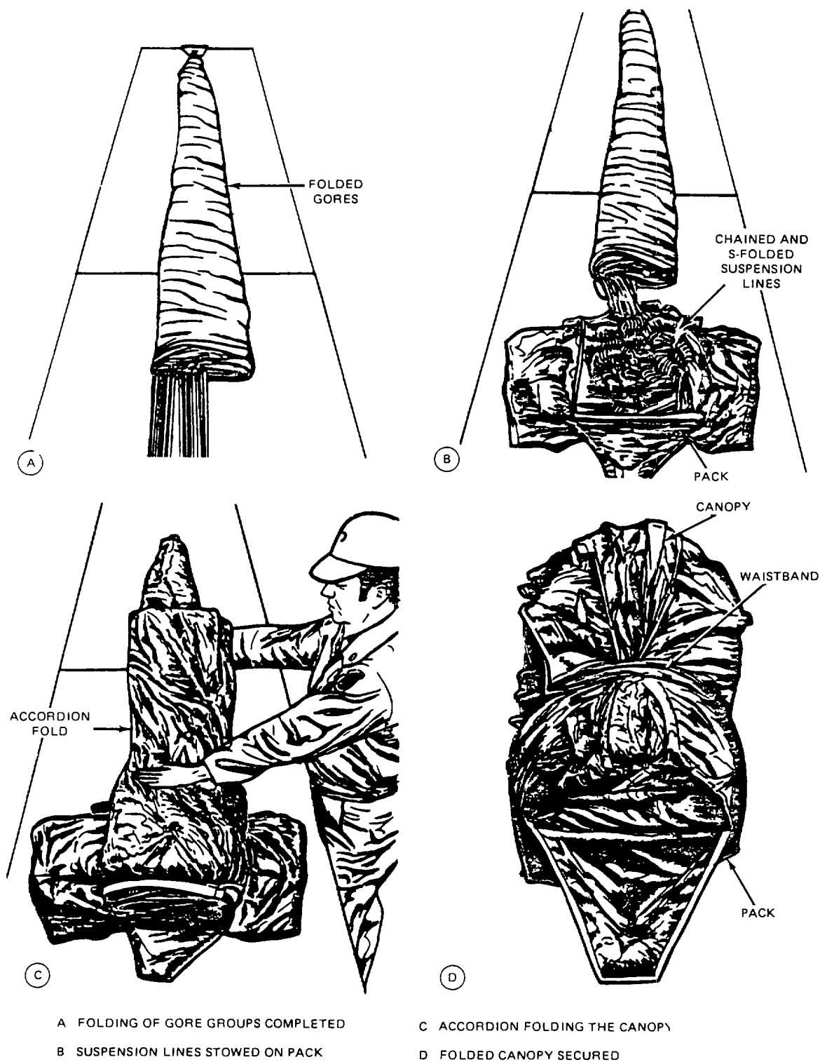
Figure 2-135. Accordion Folding a Parachute Canopy Assembly.
