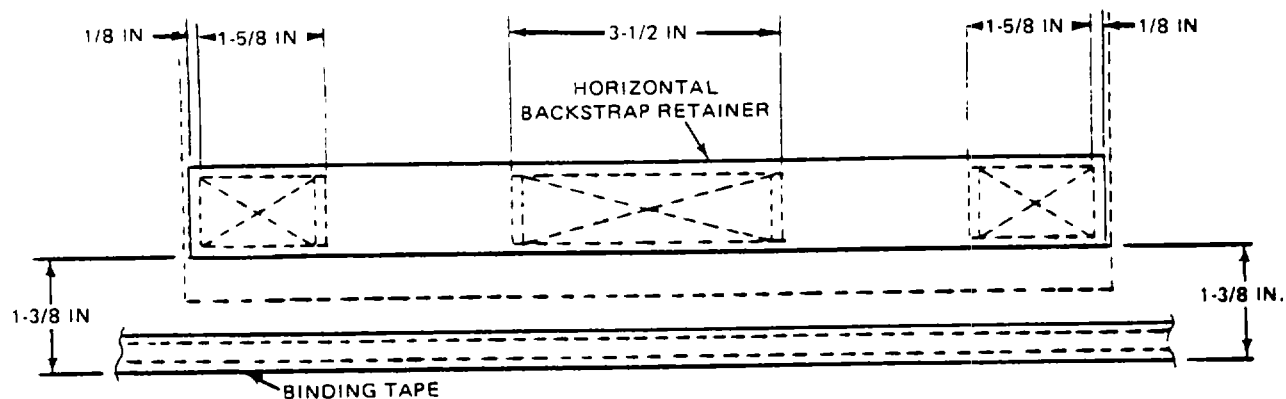
Figure 2-121. Installation of Horizontal Backstrap Retainer.
