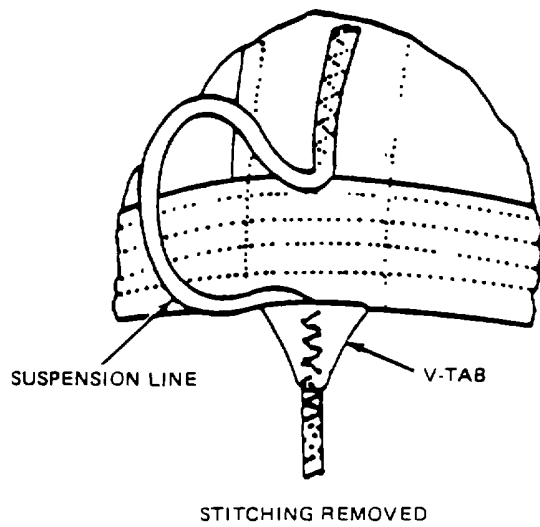
Figure 2-86. Lower Lateral Band Splicing - Damage Between Radial Seams.
