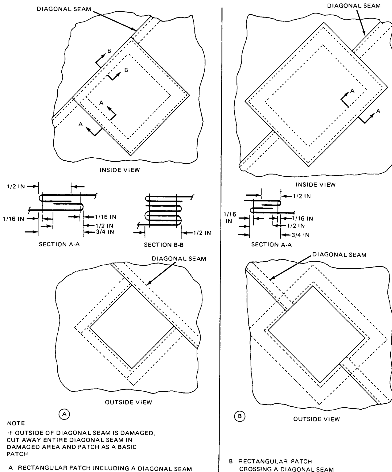
Figure 2-77. Common Miscellaneous Canopy Patches (Sheet 1 of 6).
