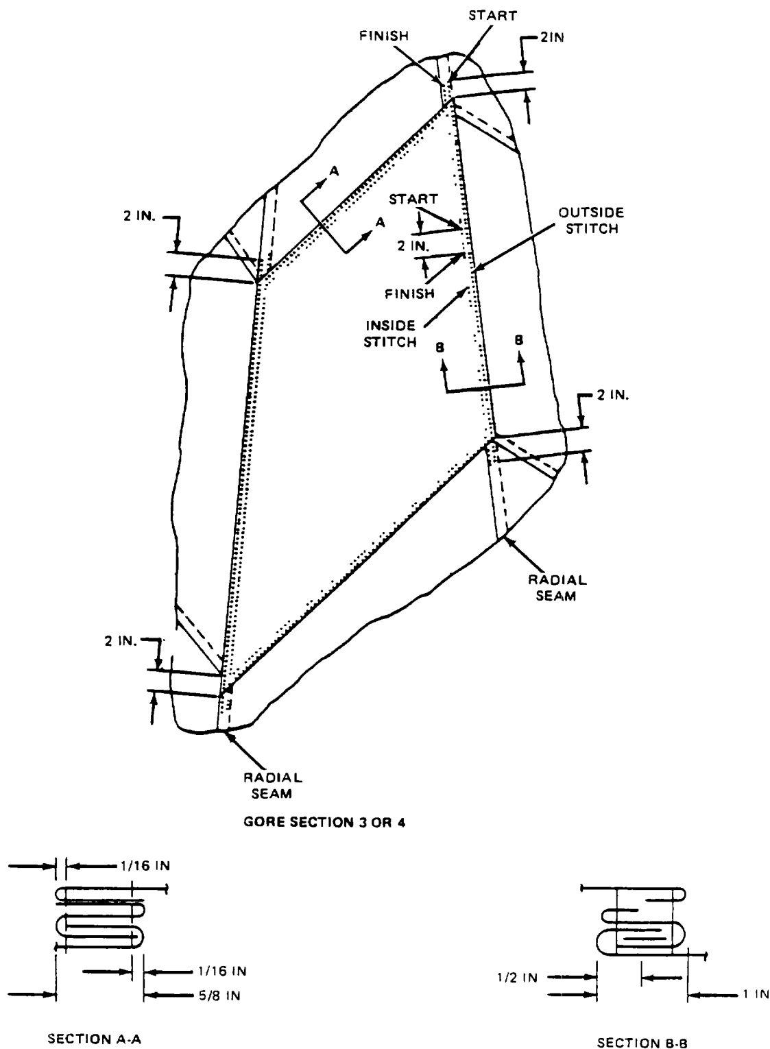
Figure 2-81. Replacing Gore Section 3 or 4.
