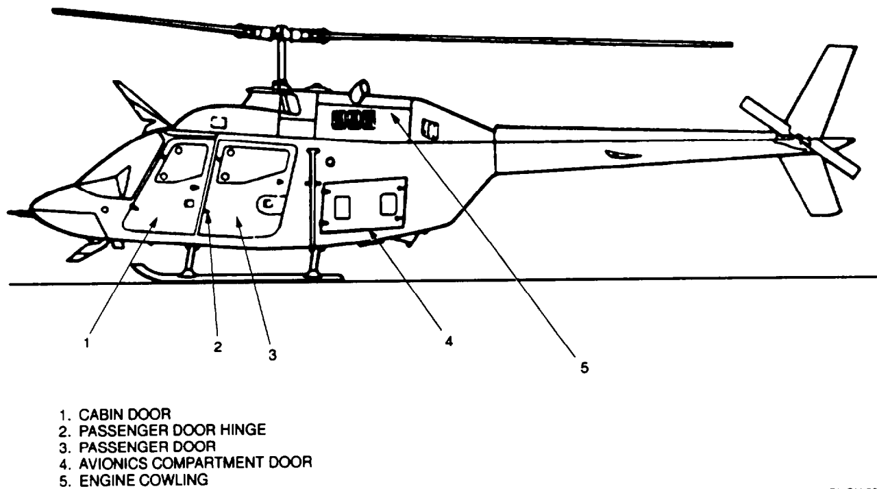
Figure 4-2. Forward and Aft Fuselage Sections
