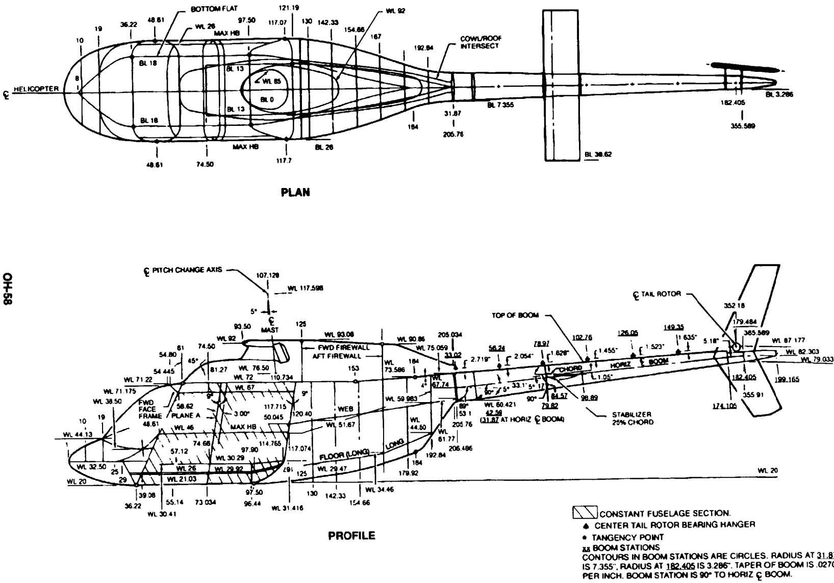
Figure 1-3. Stations, Water Lines, Butt Lines
