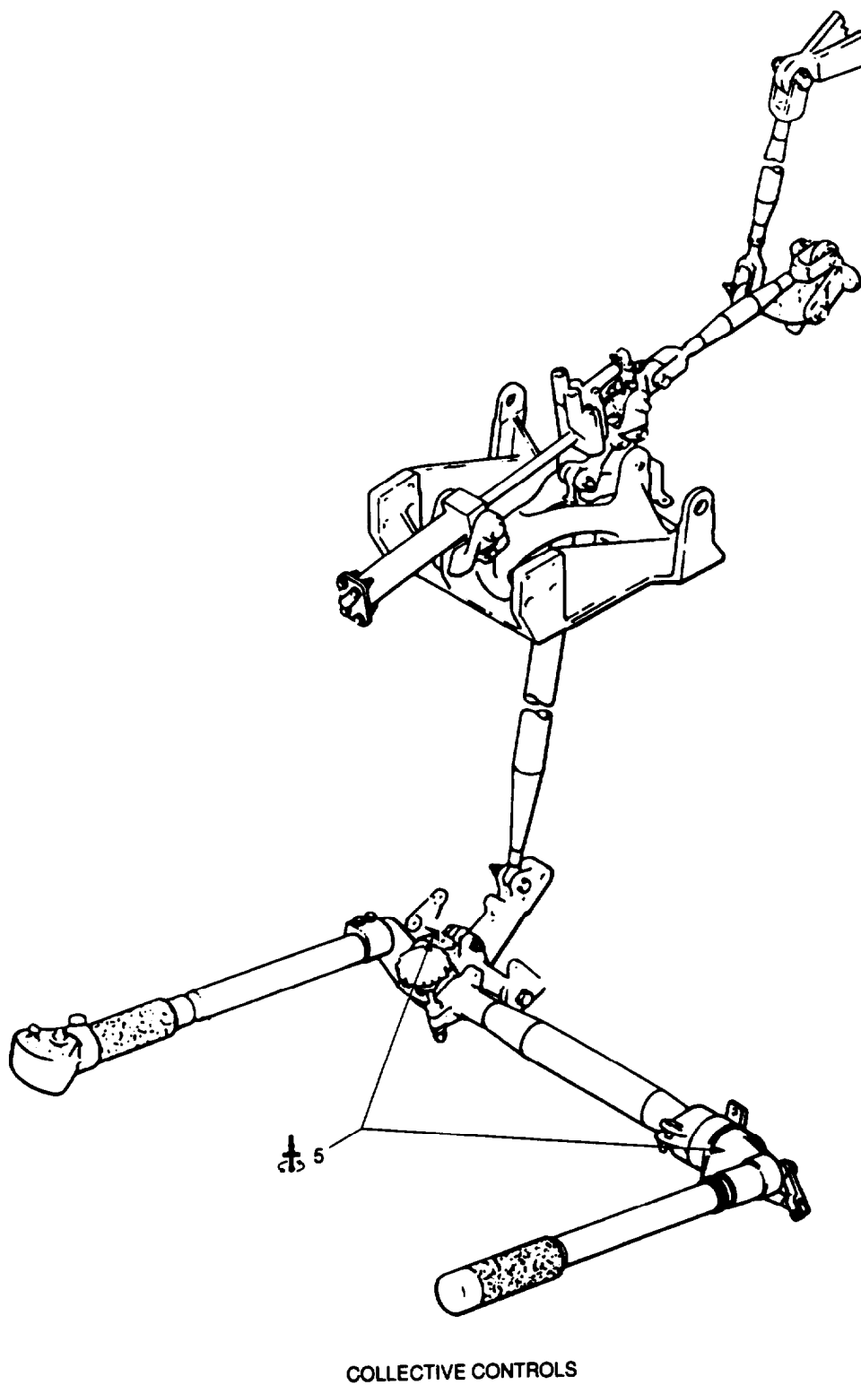
Figure 6-1. Flight Control Group (Sheet 2 of 3)
