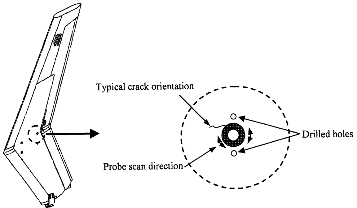
Figure 4-18. Tail Fin Attach Points.
