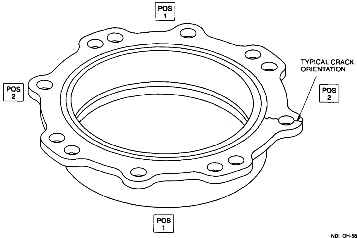
Figure 3-20. Bearing Liner
