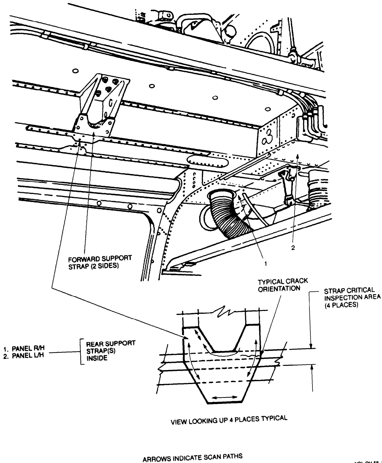
Figure 4-14. Transmission Support Straps
