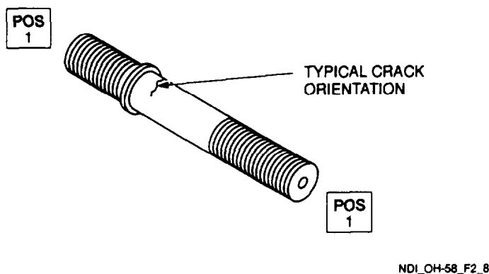
Figure 2-8. Main Rotor Blade Latch Retainer Bolt
