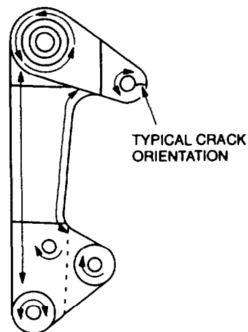
LEVER
