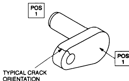
Figure 2-19. Swashplate and Support Assembly Pin
