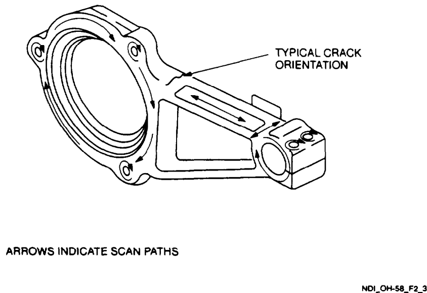
Figure 2-3. Main Rotor Pitch Horn
