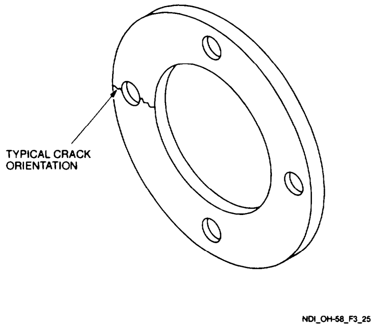
Figure 3-25. Disc Assembly
